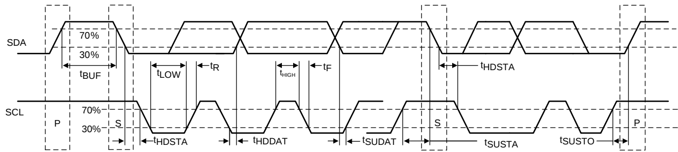
图 9. I²C Timing Diagram Definitions
