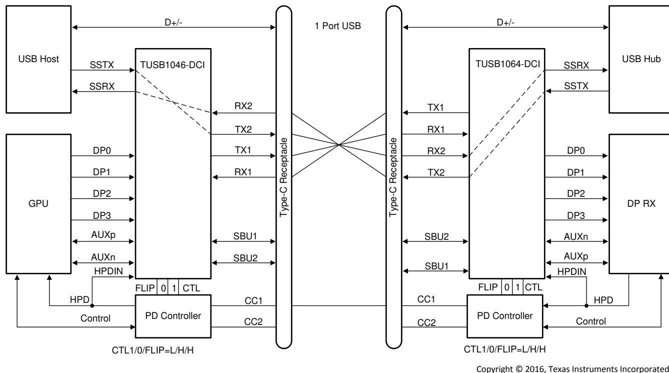
Figure 29. USB3.1 Only – No Flip (CTL1 = L, CTL0 = H, FLIP = L)
