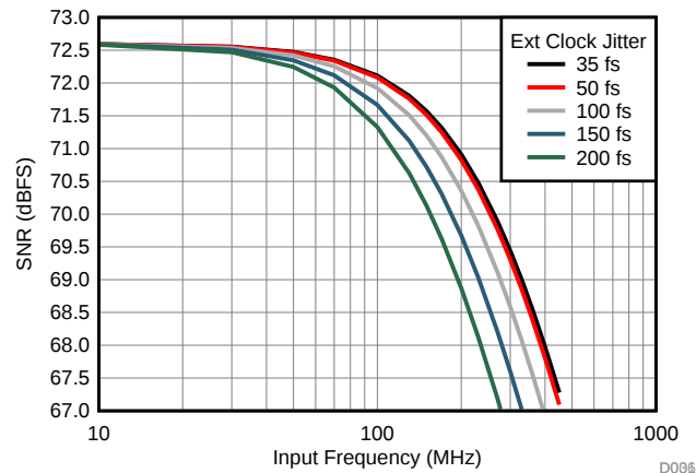
图 48. SNR vs Frequency for Different Clock Jitter
