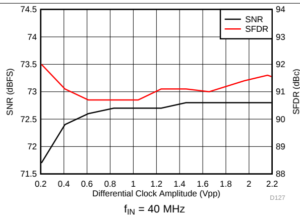
图 27. Performance vs Clock Amplitude
