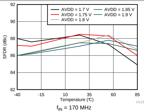
图 23. Spurious-Free Dynamic Range vs AVDD Supply and Temperature
