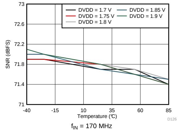
图 26. Signal-to-Noise Ratio vs DVDD Supply and Temperature
