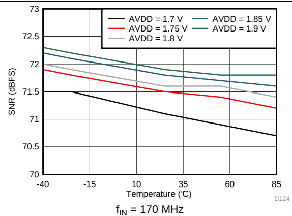
图 24. Signal-to-Noise Ratio vs AVDD Supply and Temperature
