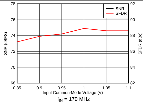
图 22. Performance vs Input Common-Mode Voltage
