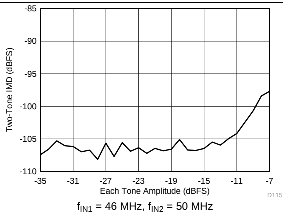
图 15. Intermodulation Distortion vs Input Amplitude
