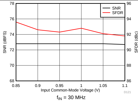
图 21. Performance vs Input Common-Mode Voltage
