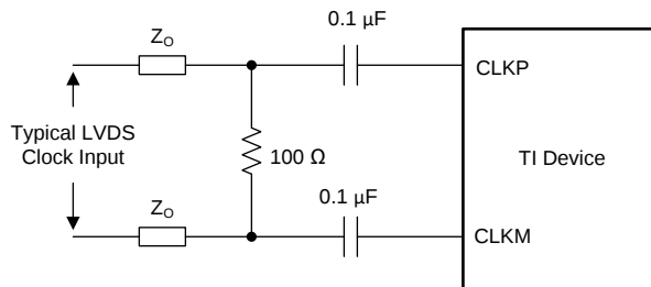
图 44. LVDS Clock Driving Circuit
