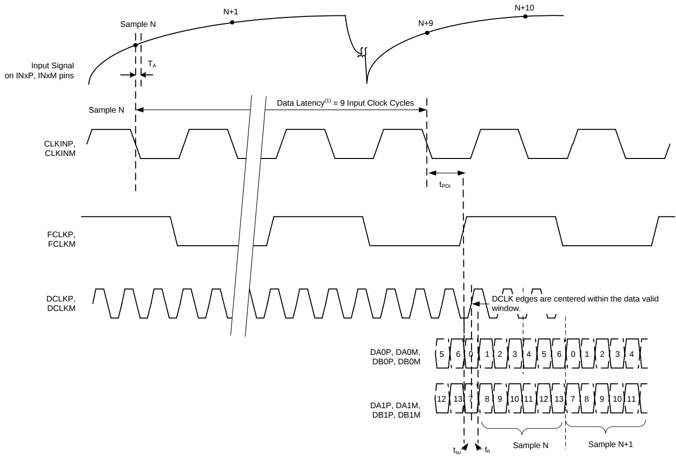
图 42. Latency Diagram
