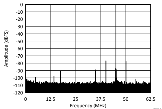
图 33. Power-Supply Rejection Ratio Spectrum
