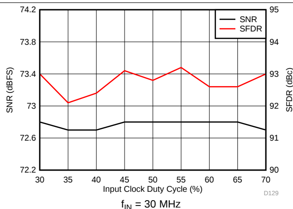
图 29. Performance vs Clock Duty Cycle
