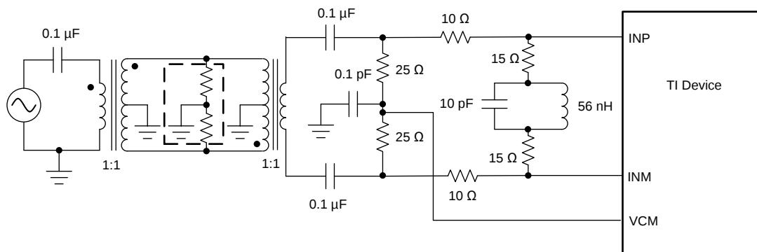
图 87. Driving Circuit for Mid-Range Input Frequencies ( 100 \text{ MHz} < f_{\text{IN}} < 230 \text{ MHz} )
