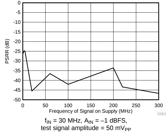
图 32. Power-Supply Rejection Ratio vs Test Signal Frequency
