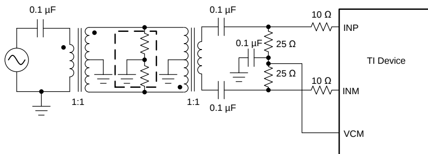
图 89. Driving Circuit for High input Frequencies ( f_{IN} > 230 MHz)
