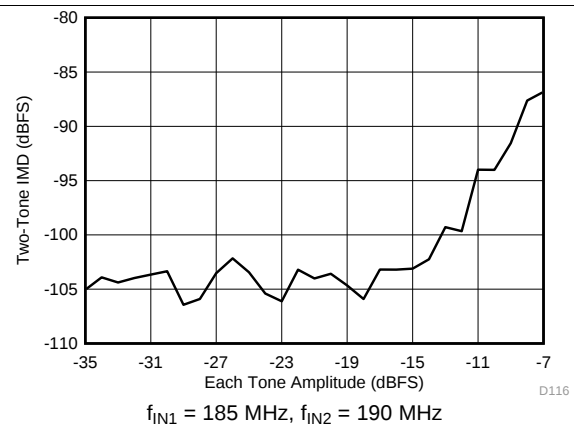
图 16. Intermodulation Distortion vs Input Amplitude
