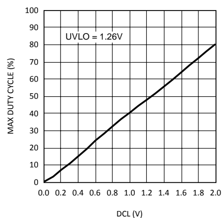
Figure 12. Max Duty Cycle vs DCL
