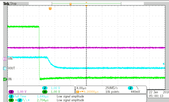
Figure 20. Fall Time ( t_F ) at V_{IN} = 1 \text{ V}
