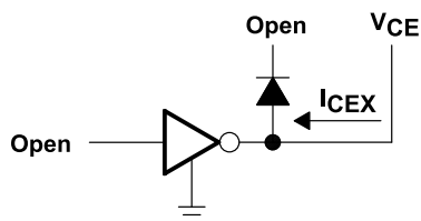
Figure 6. I_{CEX}
