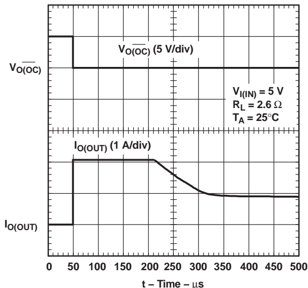
Figure 15. 2.6- \Omega Load Connected to an Enabled TPS2021 Device
