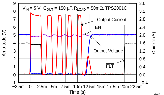
Figure 22. TPS2001C Pulsed Output Short
