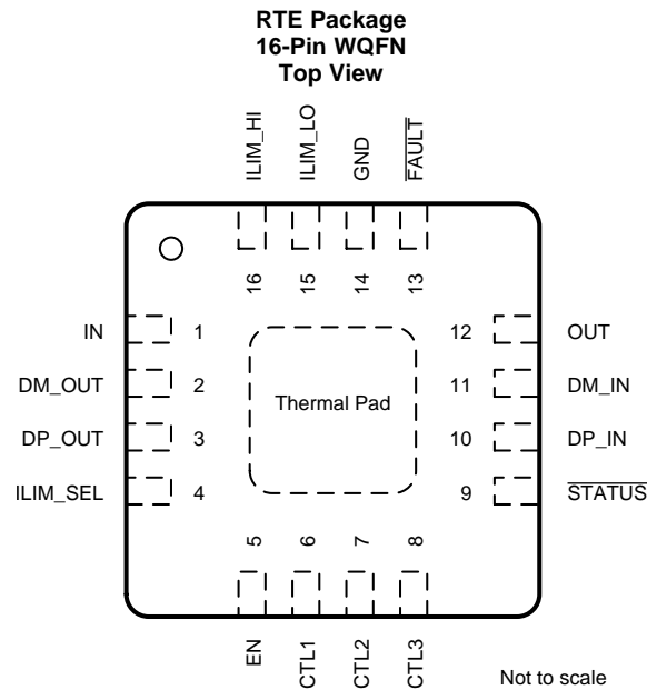
Pin Functions
