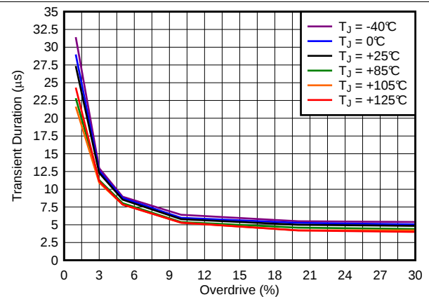
图 17. Minimum Transient Duration vs Overdrive (VDD = 5.5 V)
