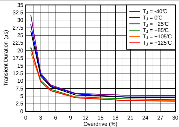
图 16. Minimum Transient Duration vs Overdrive (VDD = 1.5 V)
