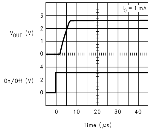
Figure 14. Enable Response
