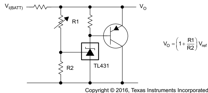
Figure 30. Precision High-Current Series Regulator
