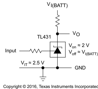
Figure 29. Single-Supply Comparator with Temperature-Compensated Threshold
