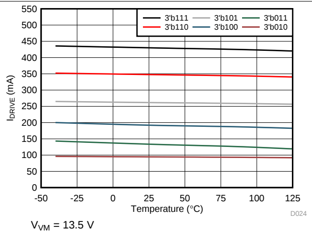
图 26. High-Side Sink Current
