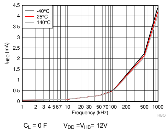
Figure 6-5. HB Operating Current
