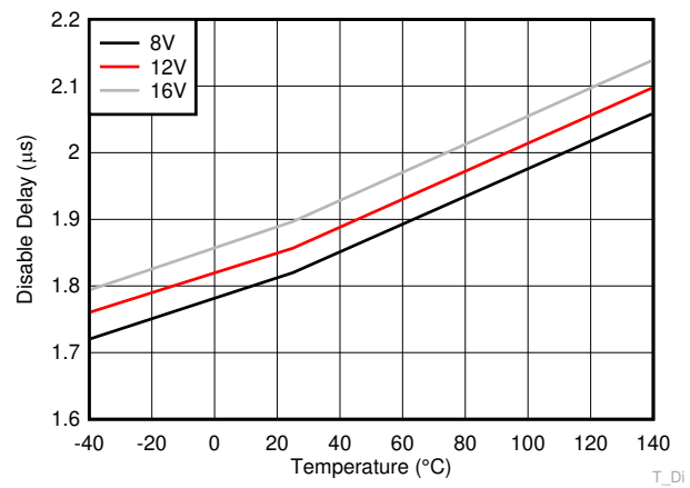
Figure 6-29. Disable Delay
