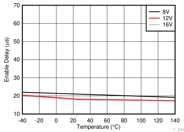
Figure 6-28. Enable Delay
