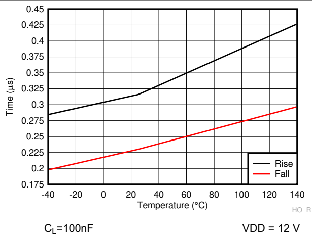
Figure 6-21. HO Rise & Fall Time
