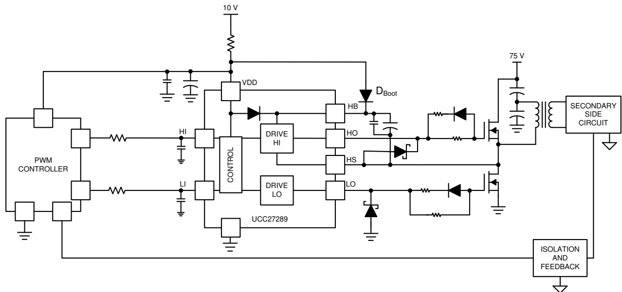
Figure 8-1. Typical Application
