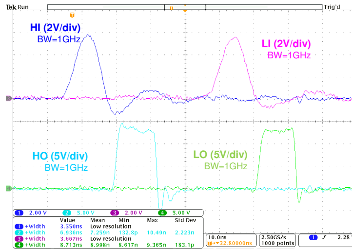
Figure 33. Input and Output Pulse Width
