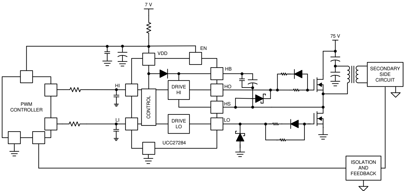
Figure 32. Typical Application
