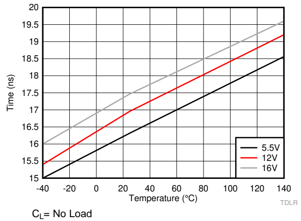
Figure 30. LO Rising Propagation Delay (TDLRR)
