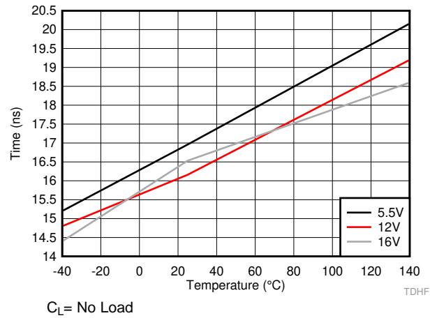
Figure 29. HO Falling Propagation Delay (TDHFF)
