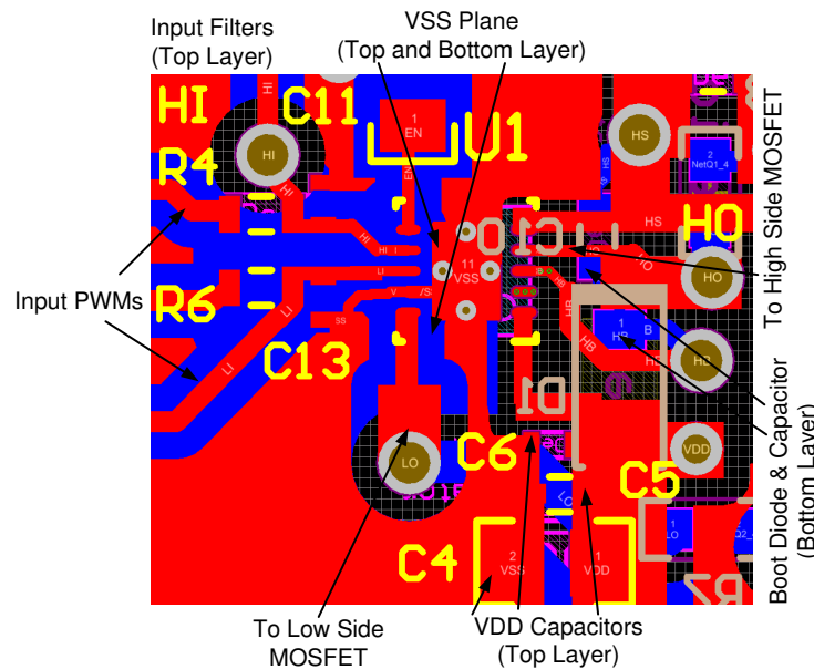
Figure 41. Layout Example
