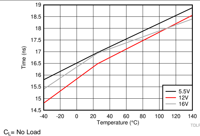
Figure 31. LO Falling Propagation Delay (TDLFF)
