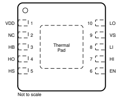
DRC Package 10-Pin VSON With Exposed Thermal Pad Top View
