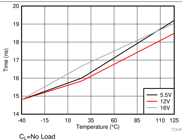
图 20. HO Rising Propagation Delay (TDHRR)
