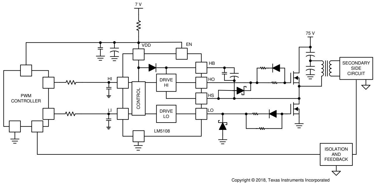
图 25. Typical Application
