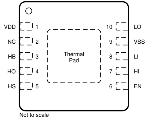
Pin Functions
