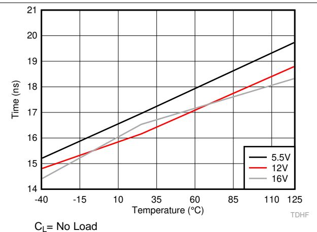
图 21. HO Falling Propagation Delay (TDHFF)
