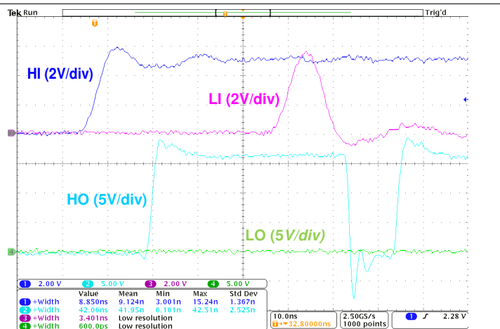
图 32. Shoot-through Protection or Interlock
