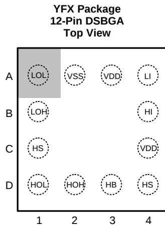
Pin Functions
