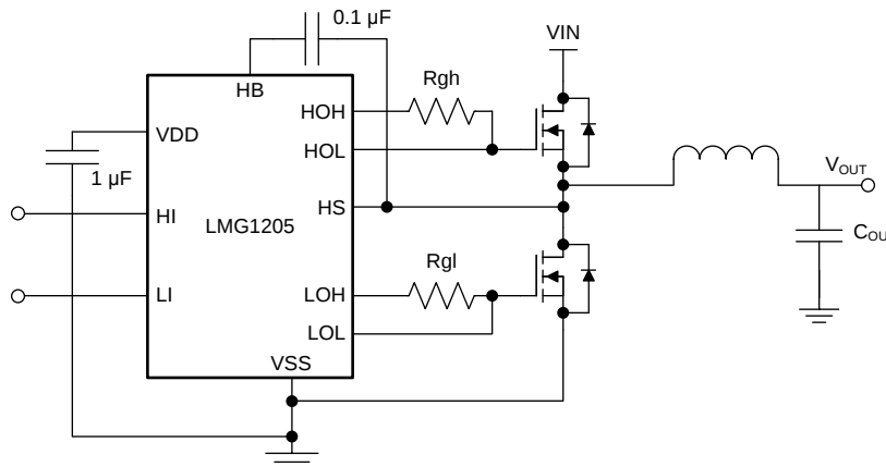
Figure 16. Application Circuit
