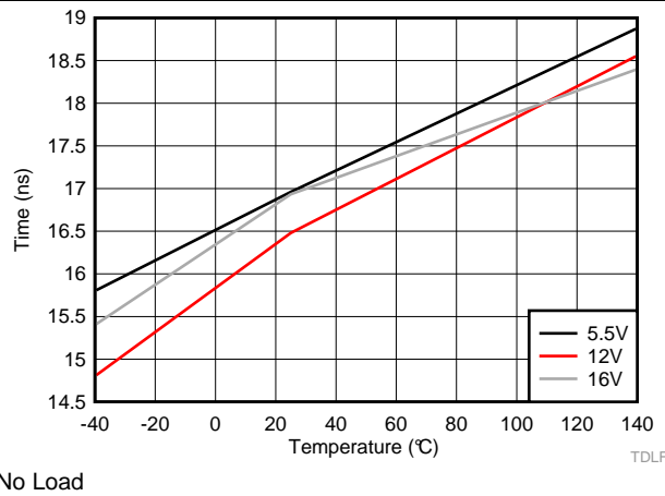
图 32. LO Falling Propagation Delay (TDLFF)
