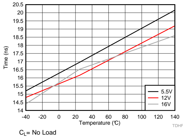
图 30. HO Falling Propagation Delay (TDHFF)
