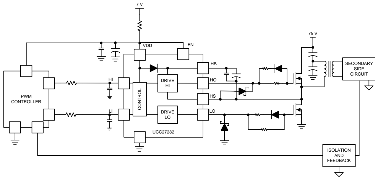
图 34. Typical Application
