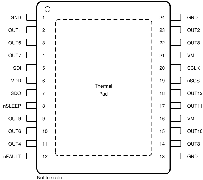
Pin Functions—DRV8912-Q1
