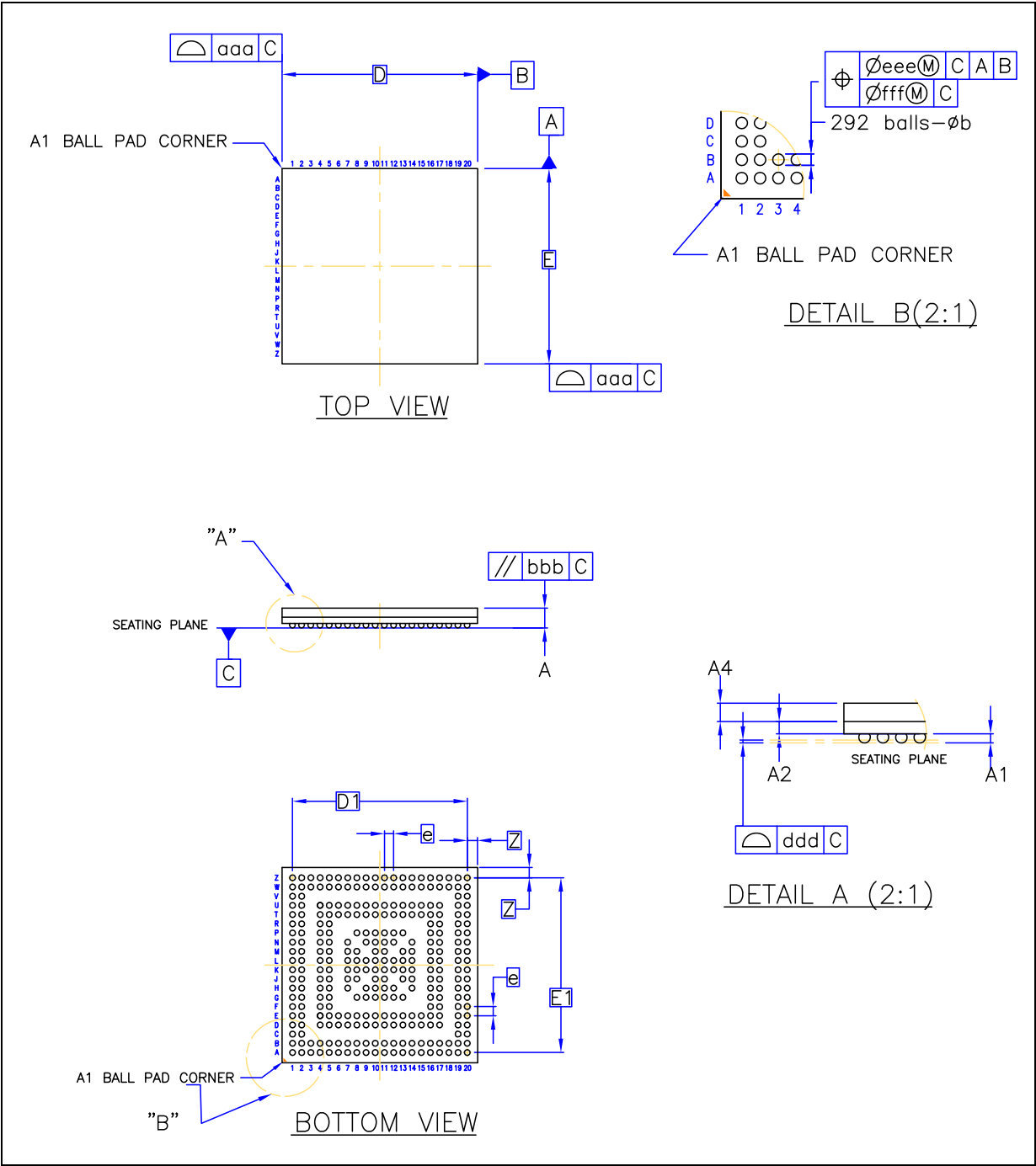
Figure 52. FPBGA292 package outline
