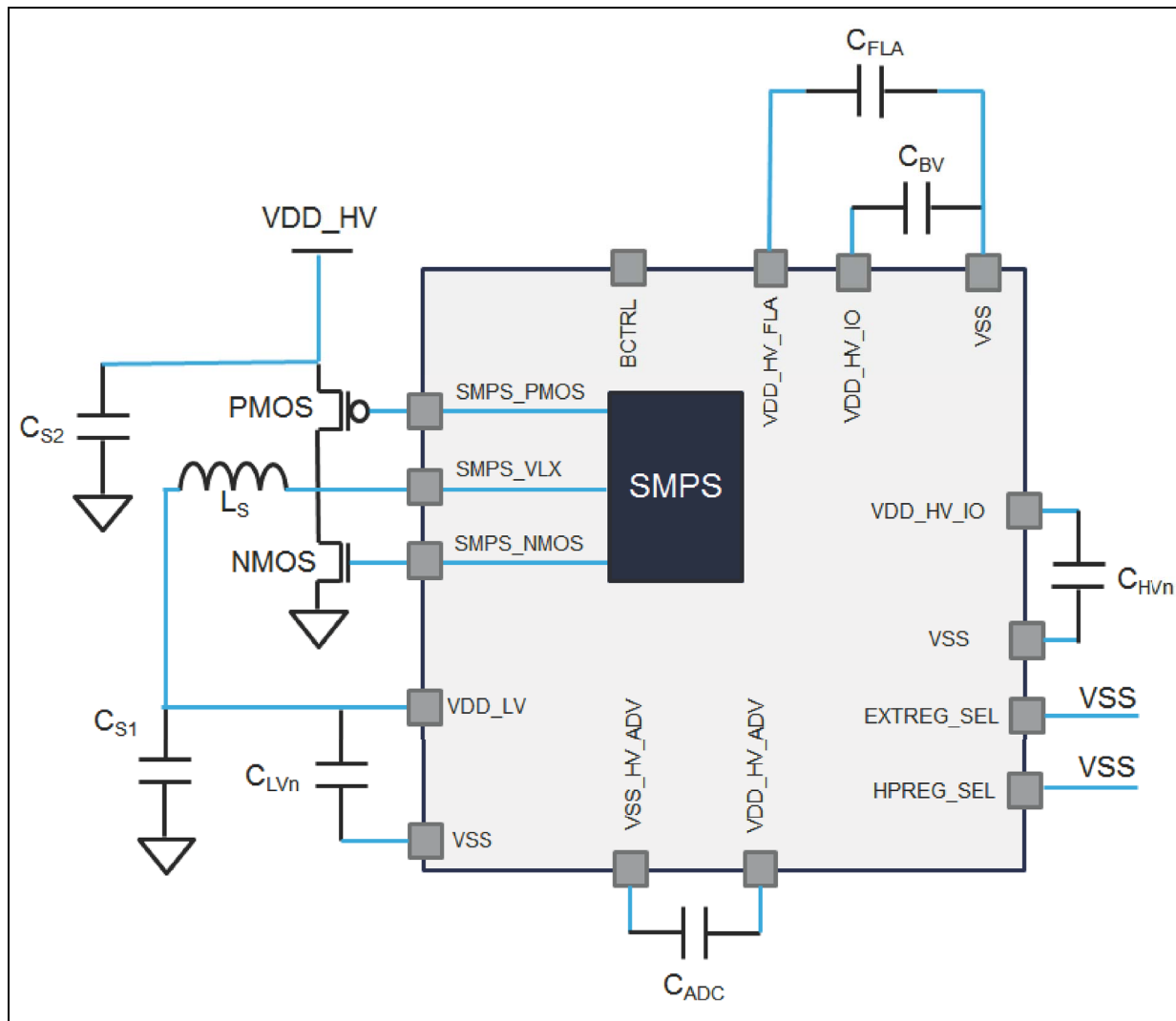
Figure 14. SMPS Regulator Mode
