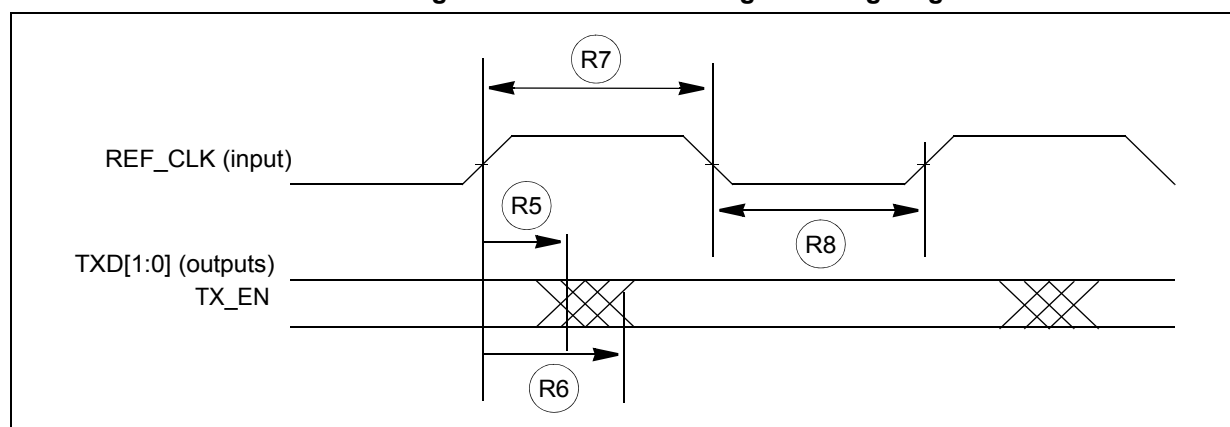
Figure 42. RMII transmit signal timing diagram
