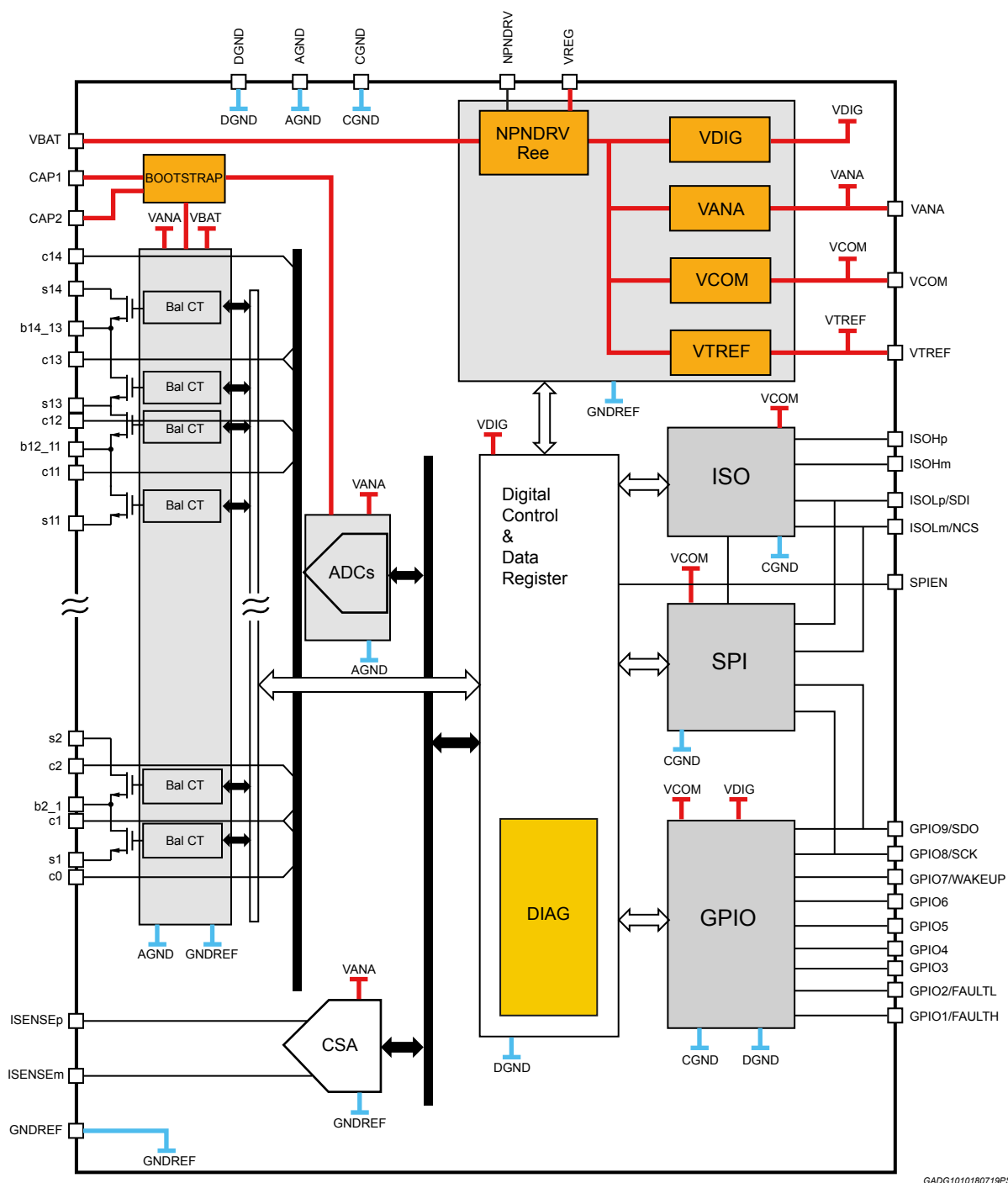
Figure 2. Block diagram
