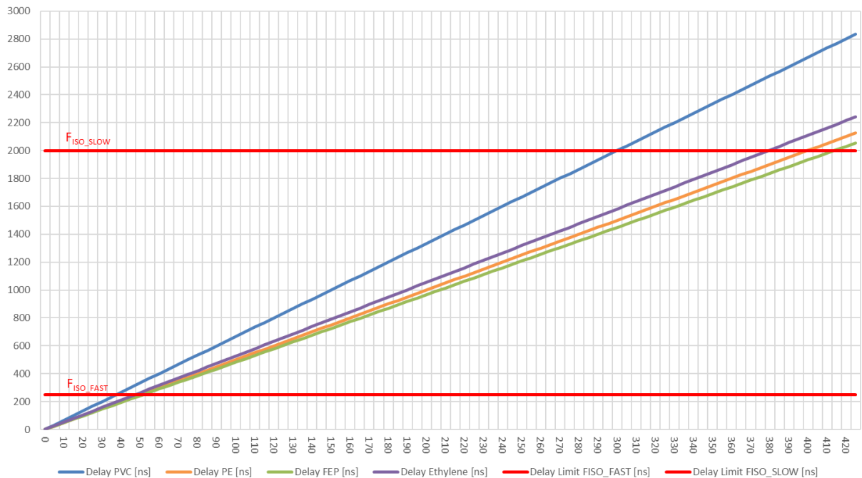
Figure 54. Maximum wire length according to wire insulator and operating frequency
