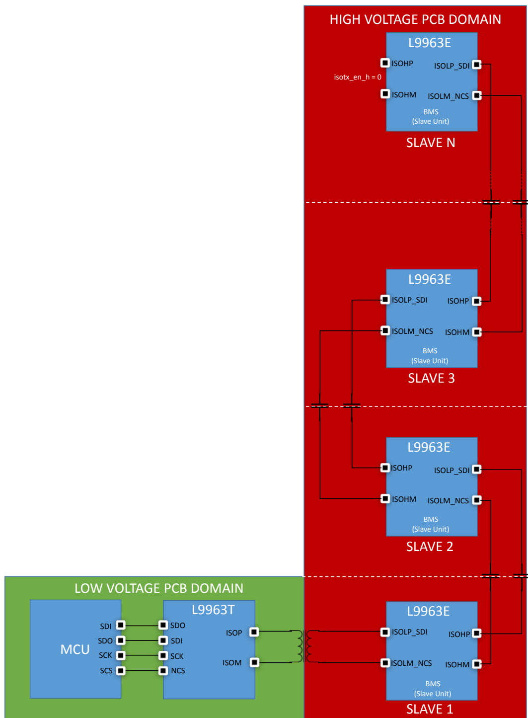
Figure 50. Centralized BMS
