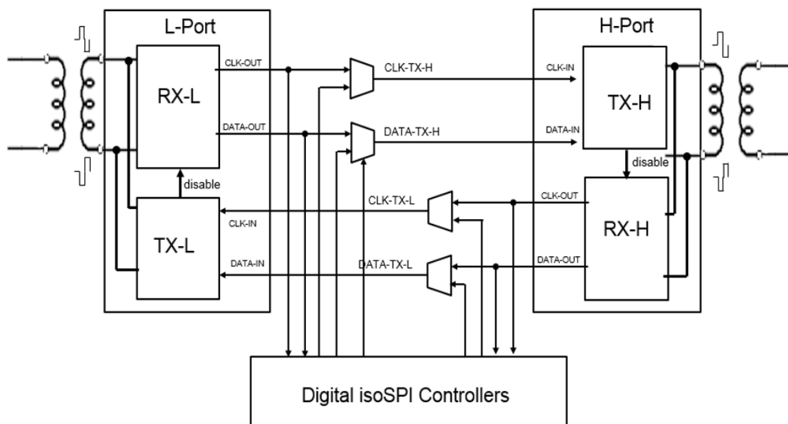
Figure 9. Isolated SPI interface
