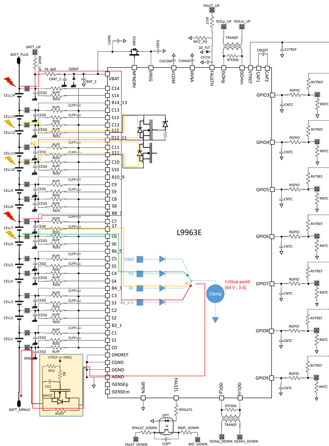
Figure 57. Hotplug paths
