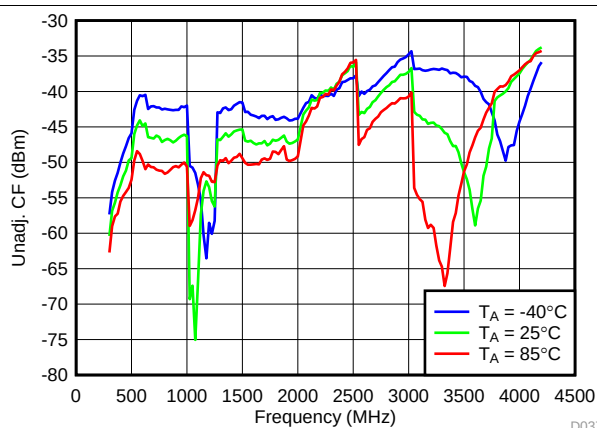
Figure 40. Unadjustable CF vs Temperature, High Gain Mode
