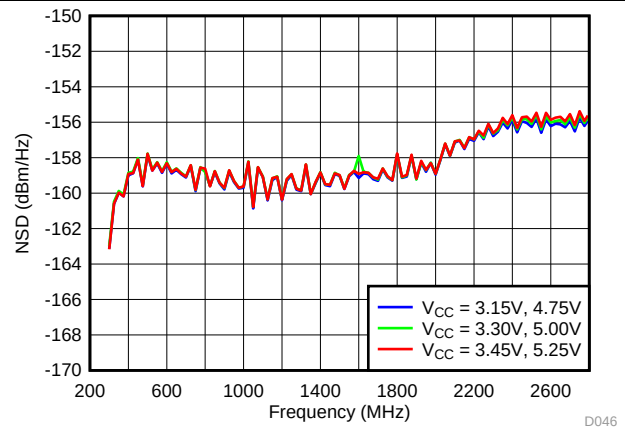
Figure 33. Noise vs Supply, Typical Operating Mode
