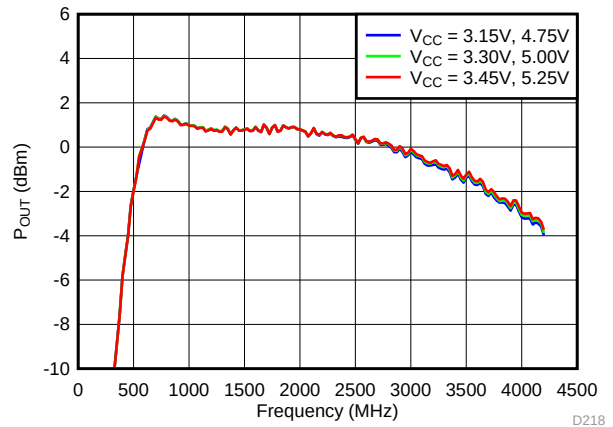
Figure 3. Total P_{OUT} vs Supply, Typical Operating Mode
