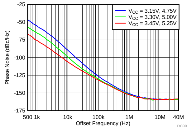
Figure 77. Open Loop Phase Noise at 450 MHz vs Supply
