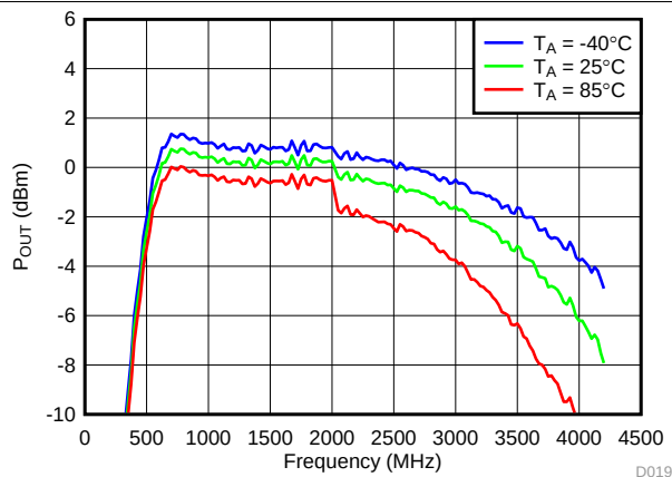
Figure 4. Total P_{OUT} vs Temperature, High Gain Mode
