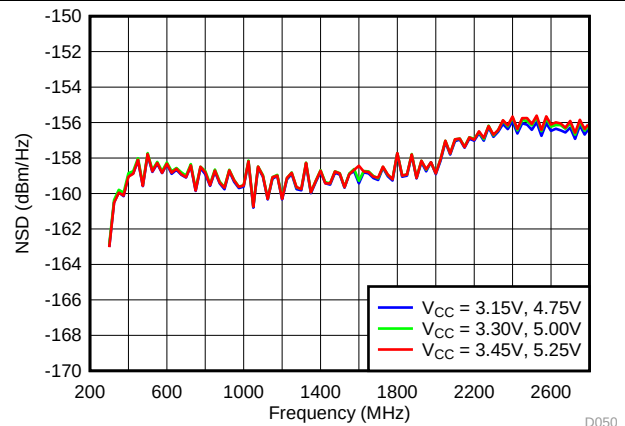
Figure 35. Noise vs Supply, High Gain Mode
