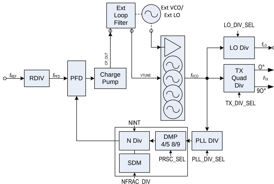
Figure 132. PLL Architecture
