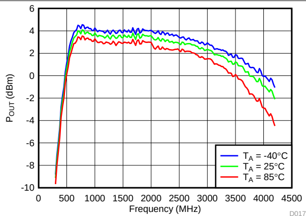
Figure 2. Total P_{OUT} vs Temperature, Typical Operating Mode
