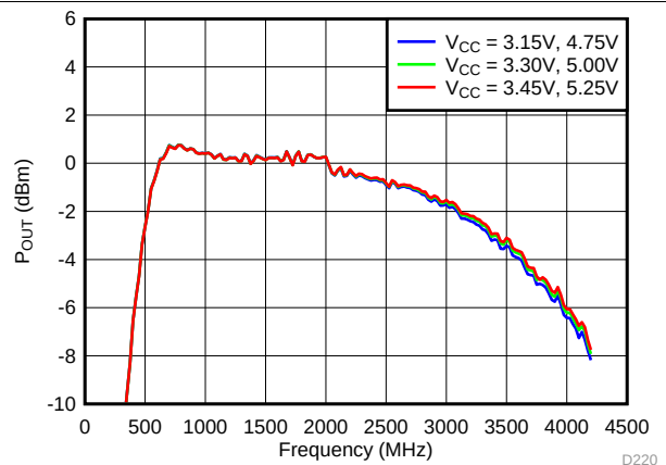
Figure 5. Total P_{OUT} vs Supply, High Gain Mode
