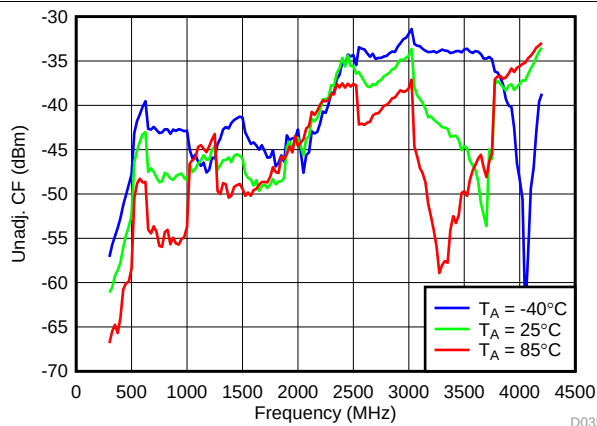
Figure 38. Unadjustable CF vs Temperature, Typical Operating Mode
