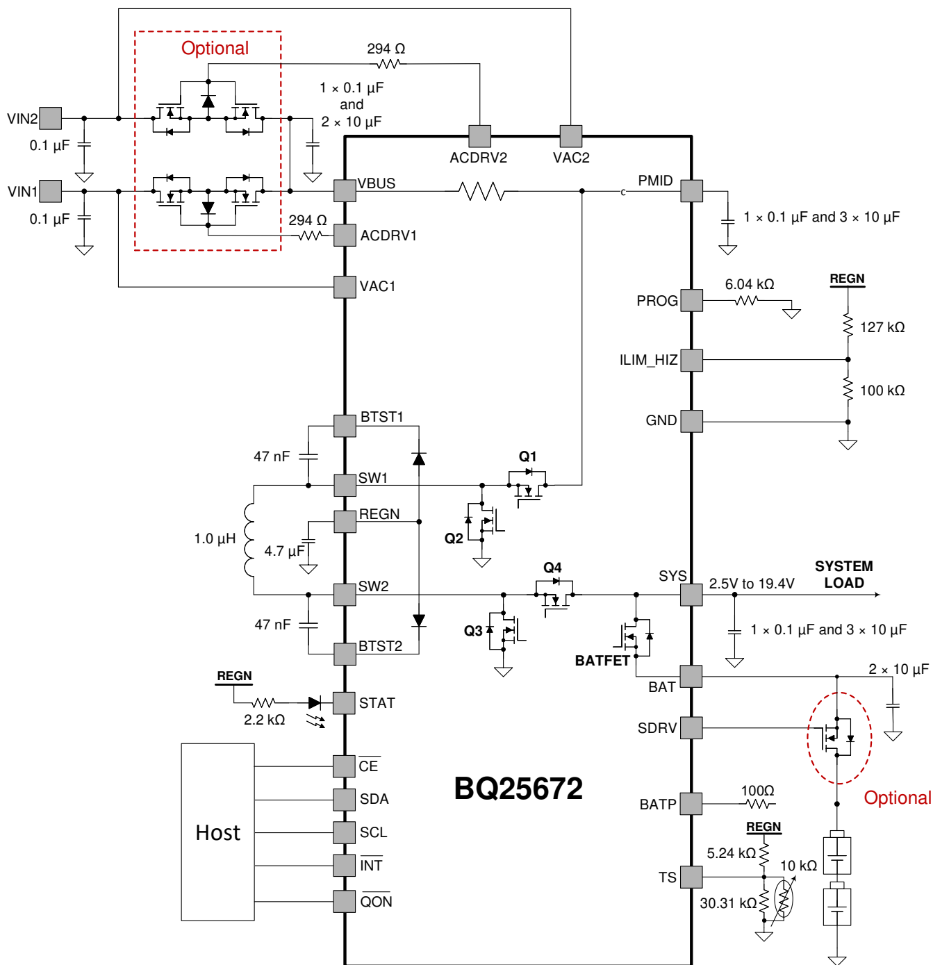
Figure 9-1. BQ25672 Application Diagram with Two Input Sources and Ship FET
