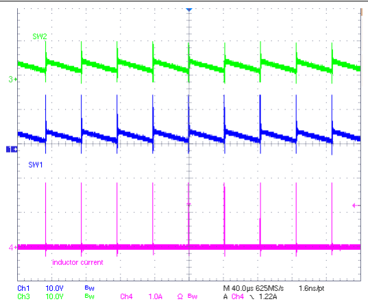
Figure 9-3. Buck Mode PFM with OOA
