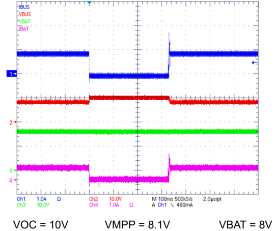
Figure 9-10. MPPT Operation Zoom
