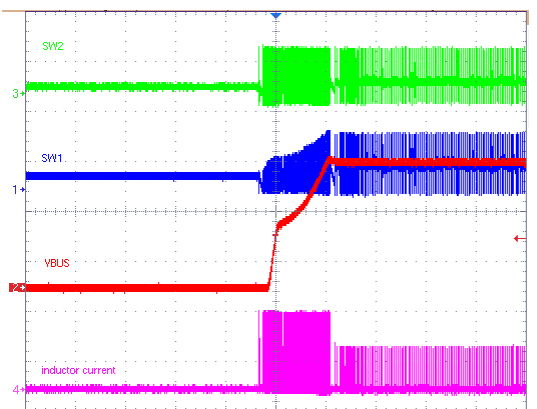
Figure 9-3. Buck Mode PFM with OOA
