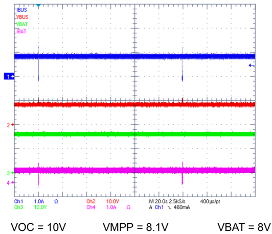
Figure 9-9. MPPT Operation
