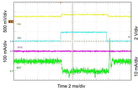
图 44. Charger On/Off Using \overline{CD}
