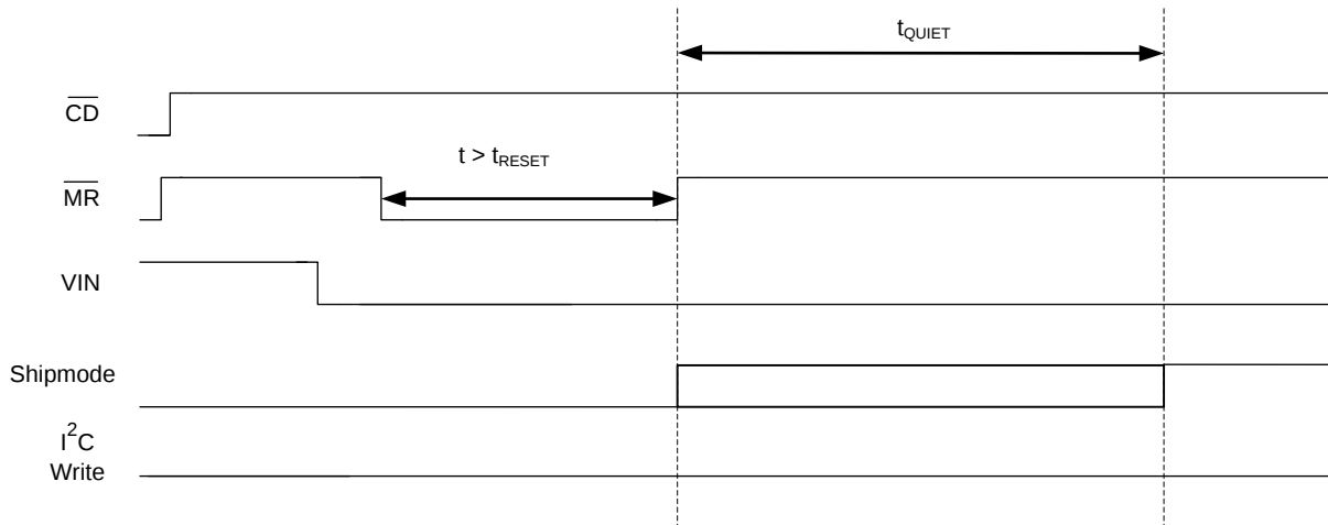
图 16. \overline{CD} , \overline{MR} and V_{IN} Sequencing for Ship Mode Entry Through Long MR button press
