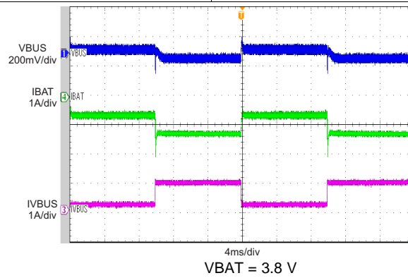
图 45. Load Transient During Supplement Mode
