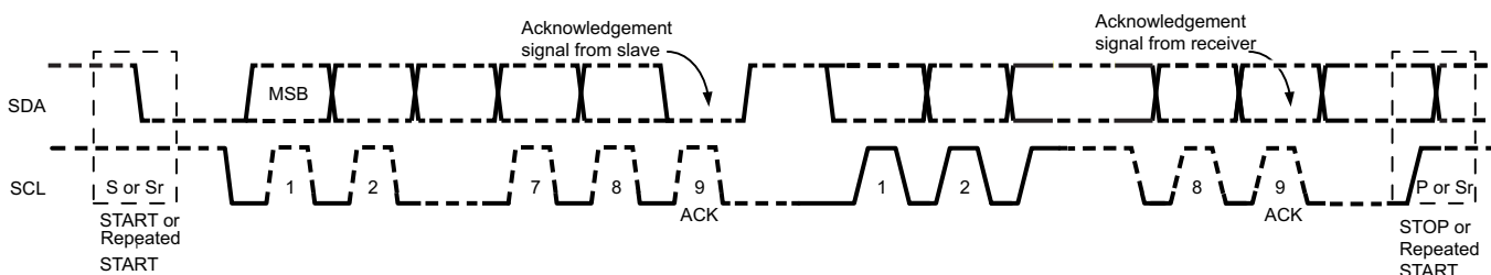
图 21. Data Transfer on the I²C Bus
