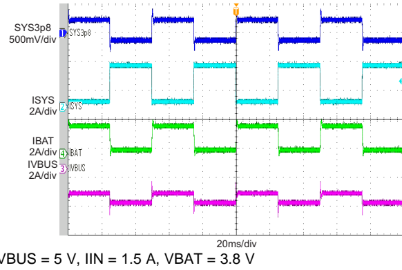
图 45. Load Transient During Supplement Mode
