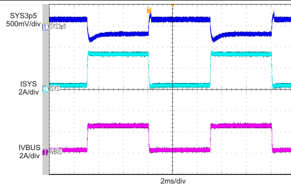
图 42. PWM Switching in Buck Mode
