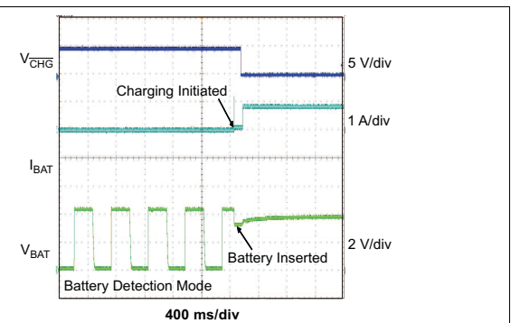
Figure 25. Battery Detection / Battery Inserted
