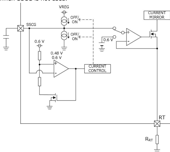
Figure 6. SSCG System Diagram
