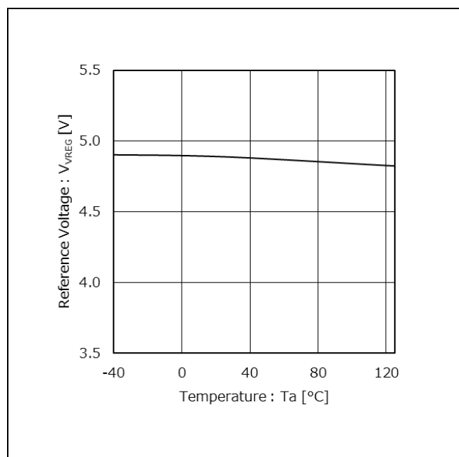
Figure 9. Reference Voltage vs Temperature ( V_{CC} = 12\text{ V} , V_{EN} = 3.3\text{ V} , V_{PWM} = 0\text{ V} )
