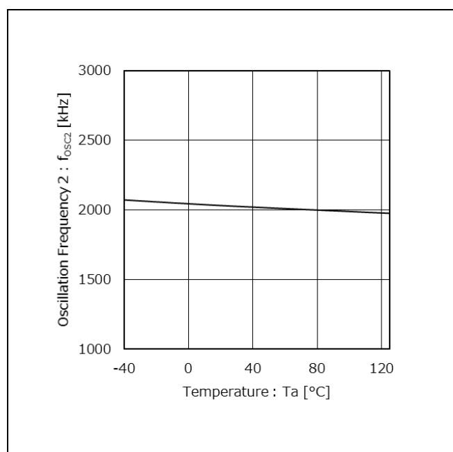
Figure 11. Oscillation Frequency 2 vs Temperature (@2000 kHz, V_{CC} = 12\text{ V} , V_{EN} = 3.3\text{ V} , R_{RT} = 3.6\text{ k}\Omega )
