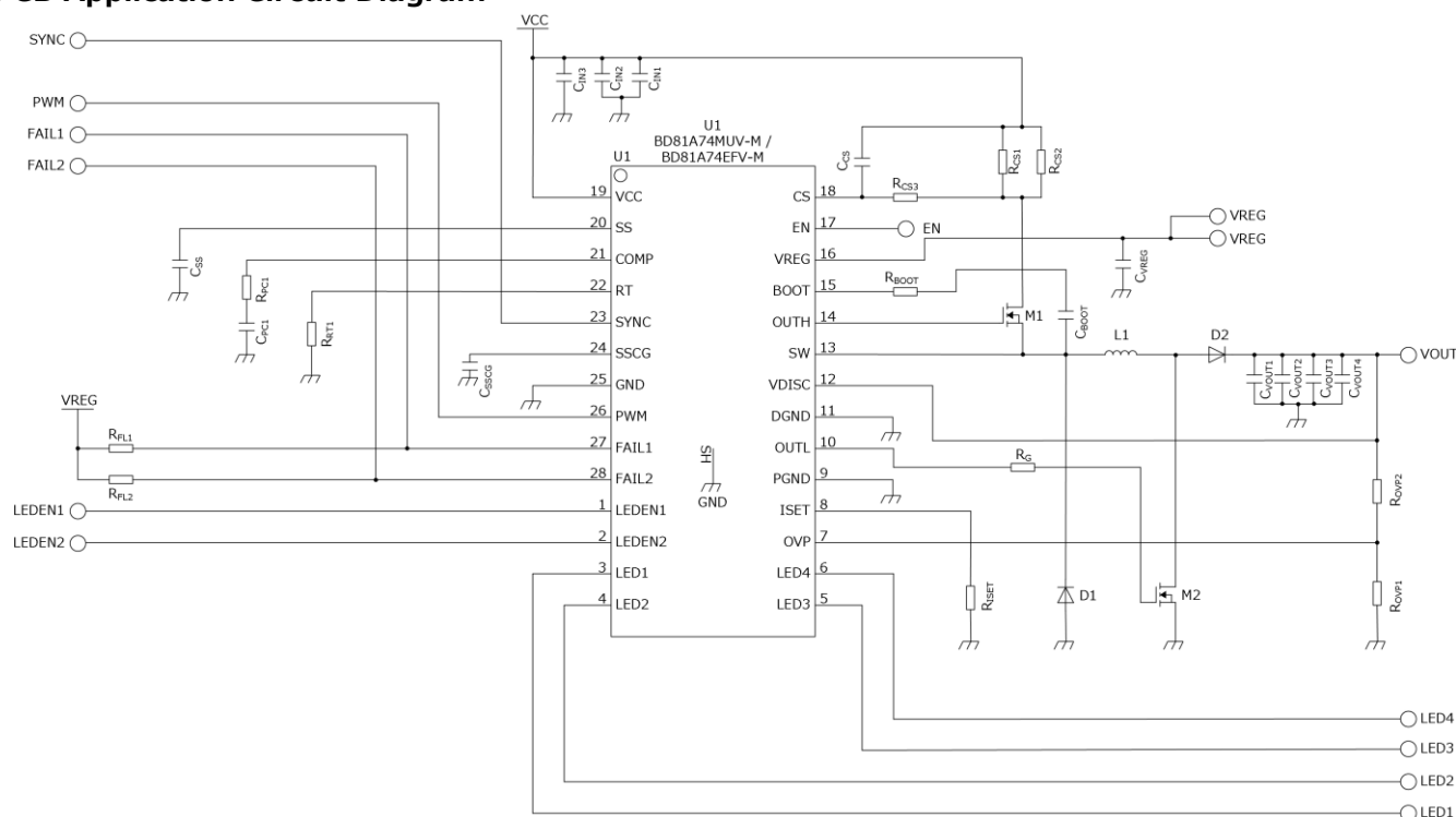
Figure 18. PCB Application Circuit
