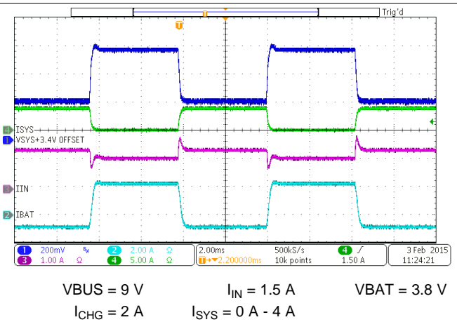
图 55. Load Transient During Supplement Mode
