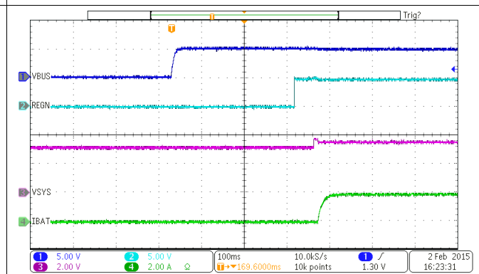
图 49. Power Up with Charge Disabled
