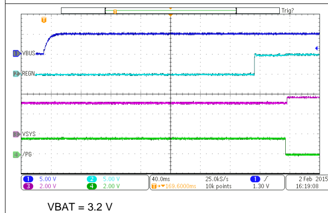
图 48. Power Up from USB100
