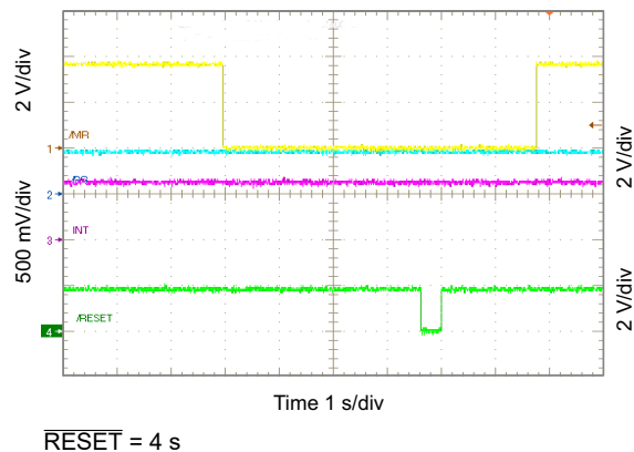
Figure 10-65. \overline{\text{RESET}} Timing
