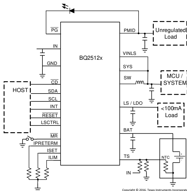
Simplified Schematic
