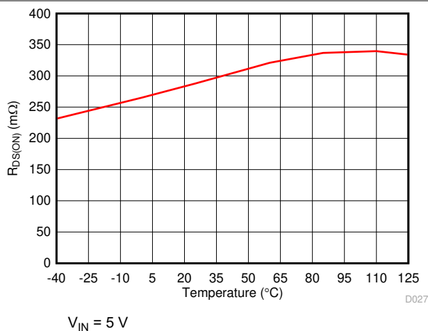
Figure 8-13. R_{DS(ON)} of Low Side MOSFET vs Temperature
