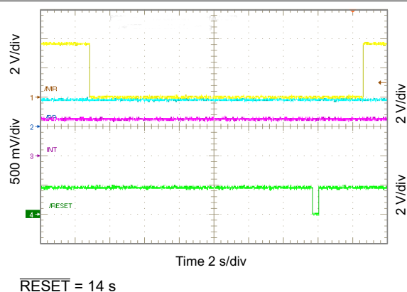
Figure 10-67. \overline{\text{RESET}} Timing
