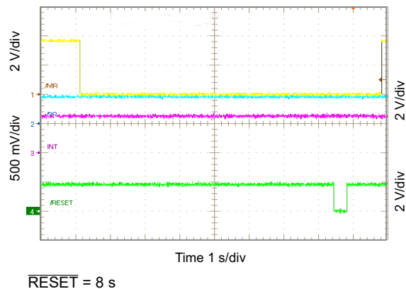
Figure 10-66. \overline{\text{RESET}} Timing
