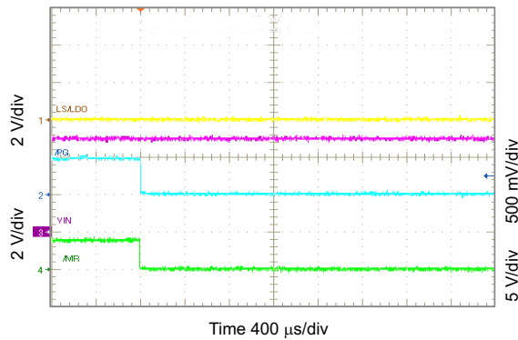
Figure 10-61. \overline{PG} Functions as Shifted \overline{MR} Output
