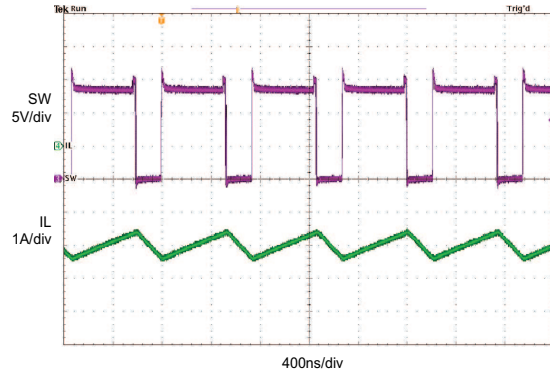
图 40. Boost Mode Switching Waveform
