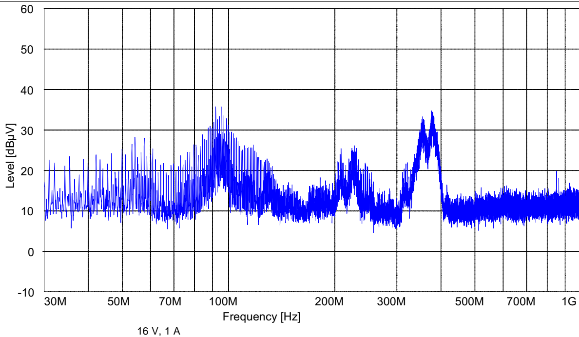
Figure 7. Typical Radiated EMI Performance Measured on EVM
