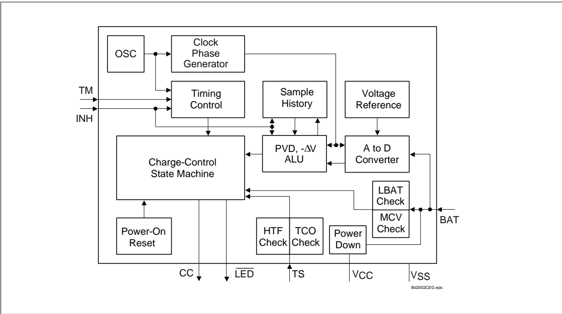
Figure 3. Block Diagram
