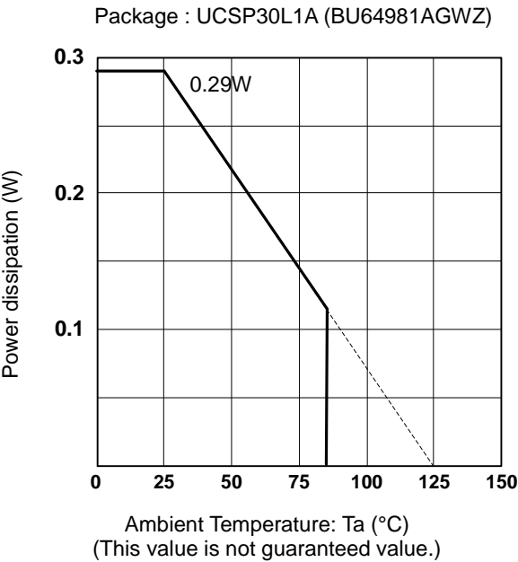
Figure 9. Power dissipation Pd (W)
