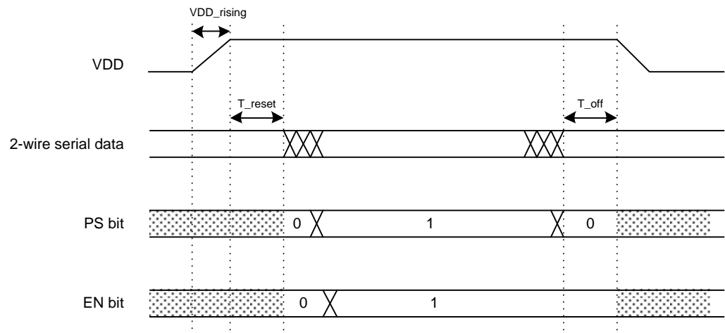
Figure 4. Timing Chart
