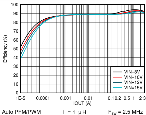
图 8-7. Efficiency vs Output Current V_{\text{OUT}} = 5 \text{ V}
