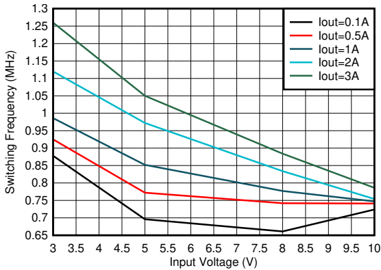
图 8-72. Switching Frequency vs Input Voltage V_{\text{OUT}} = 0.4 \text{ V}
