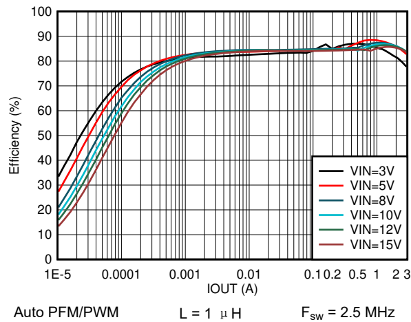
图 8-19. Efficiency vs Output Current V_{OUT} = 1.2 V
