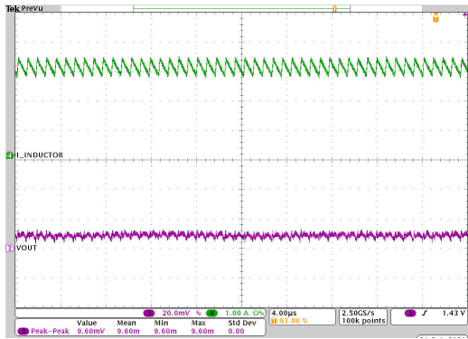
图 8-47. Output Voltage Ripple
