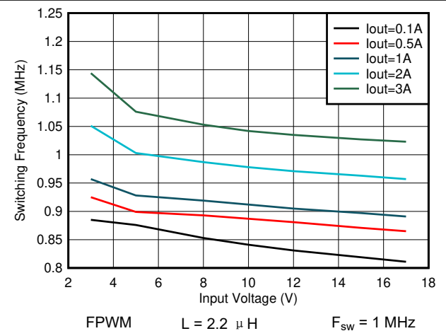
图 8-34. Switching Frequency vs Input Voltage V_{\text{OUT}} = 1.2 \text{ V}
