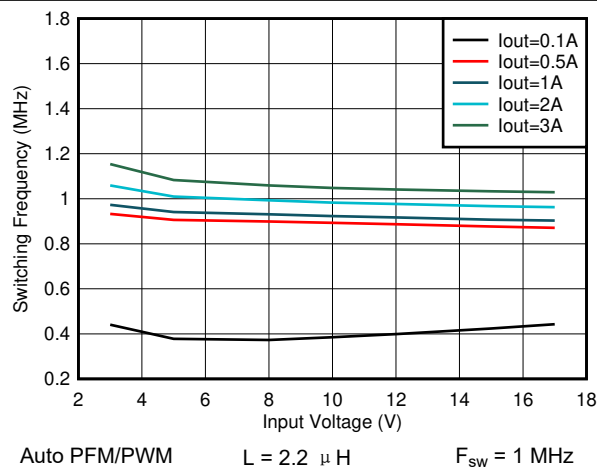
图 8-33. Switching Frequency vs Input Voltage V_{\text{OUT}} = 1.2 \text{ V}
