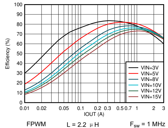
图 8-69. Efficiency vs Output Current V_{OUT} = 0.4\text{ V}
