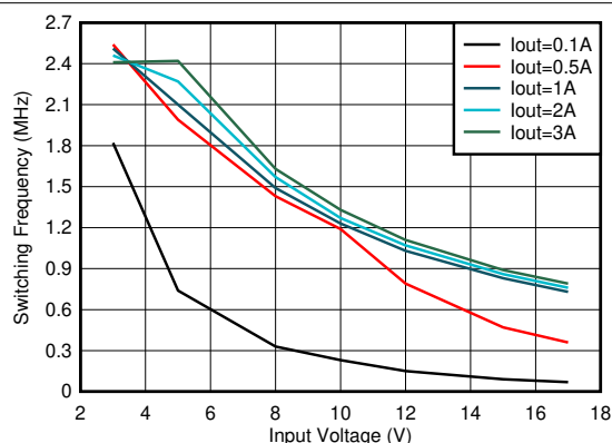
图 8-35. Switching Frequency vs Input Voltage V_{\text{OUT}} = 1.2 \text{ V}
