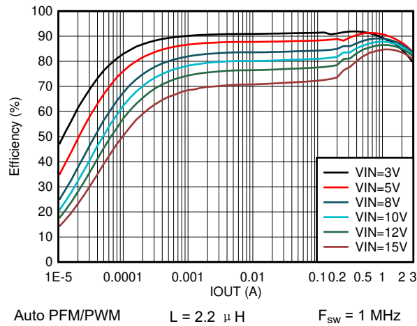
图 8-17. Efficiency vs Output Current V_{OUT} = 1.2 V
