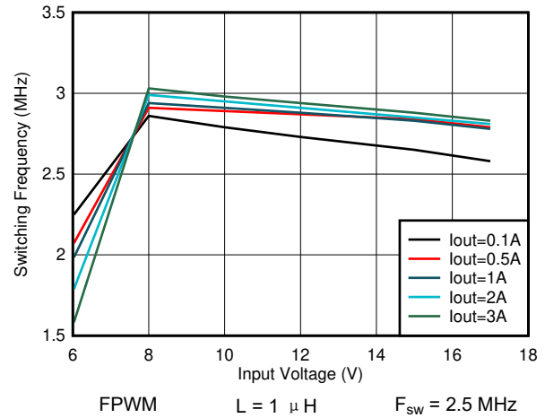
图 8-24. Switching Frequency vs Input Voltage V_{OUT} = 5 V
