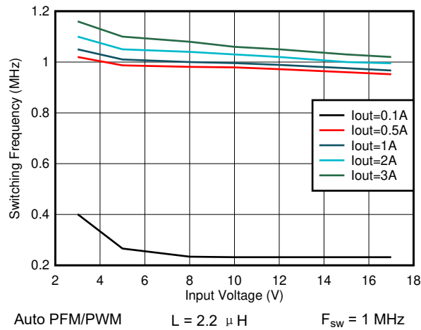
图 8-29. Switching Frequency vs Input Voltage V_{\text{OUT}} = 1.8 \text{ V}
