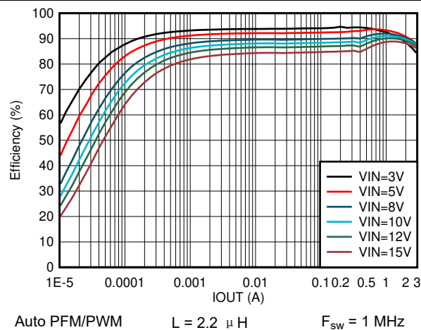
图 8-13. Efficiency vs Output Current V_{\text{OUT}} = 1.8 \text{ V}
