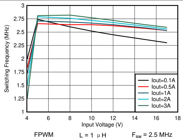
图 8-28. Switching Frequency vs Input Voltage V_{OUT} = 3.3 V
