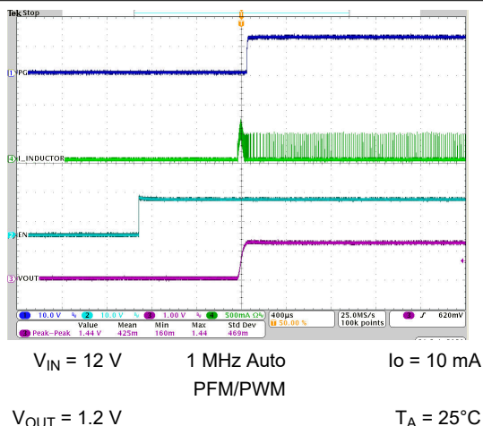
图 8-39. Start-up Timing
