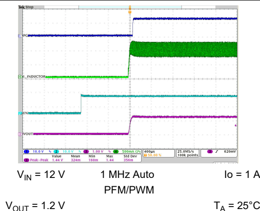
图 8-40. Start-up Timing
