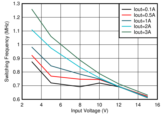
图 8-73. Switching Frequency vs Input Voltage V_{\text{OUT}} = 0.4 \text{ V}
