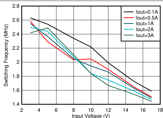
图 8-36. Switching Frequency vs Input Voltage V_{\text{OUT}} = 1.2 \text{ V}
