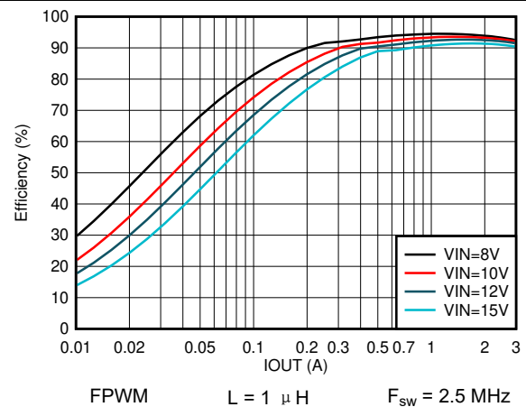
图 8-8. Efficiency vs Output Current V_{\text{OUT}} = 5 \text{ V}
