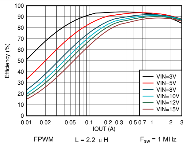
图 8-14. Efficiency vs Output Current V_{\text{OUT}} = 1.8 \text{ V}
