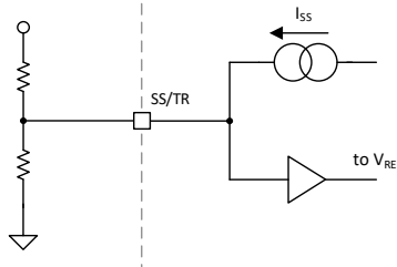
图 8-3. Tracking Operation Simplified Schematic
