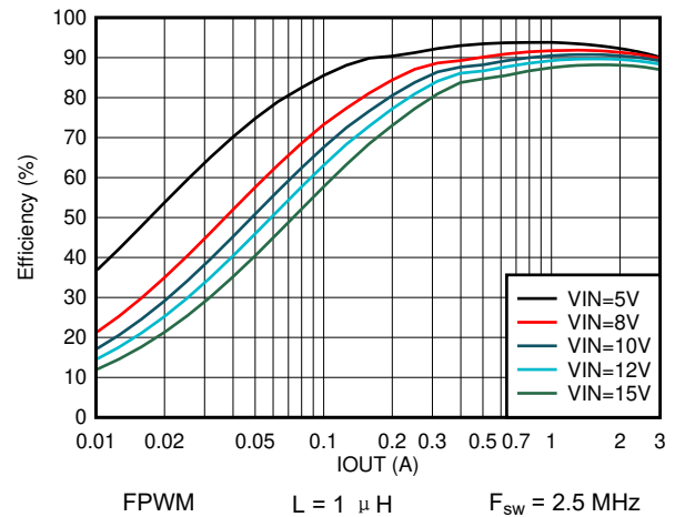
图 8-12. Efficiency vs Output Current V_{\text{OUT}} = 3.3 \text{ V}
