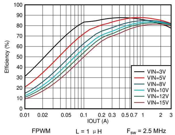
图 8-20. Efficiency vs Output Current V_{OUT} = 1.2 V
