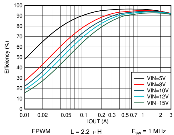
图 8-10. Efficiency vs Output Current V_{\text{OUT}} = 3.3 \text{ V}
