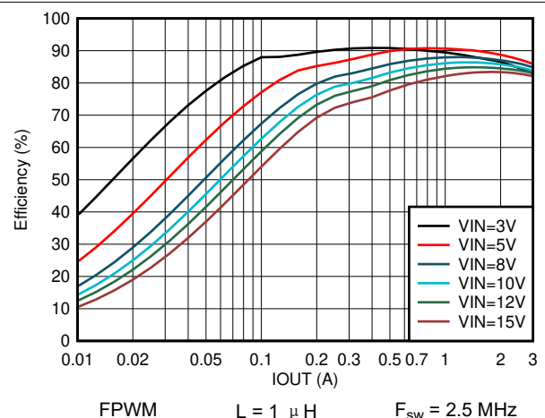
图 8-16. Efficiency vs Output Current V_{\text{OUT}} = 1.8 \text{ V}
