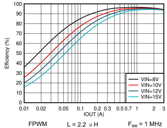
图 8-6. Efficiency vs Output Current V_{\text{OUT}} = 5 \text{ V}
