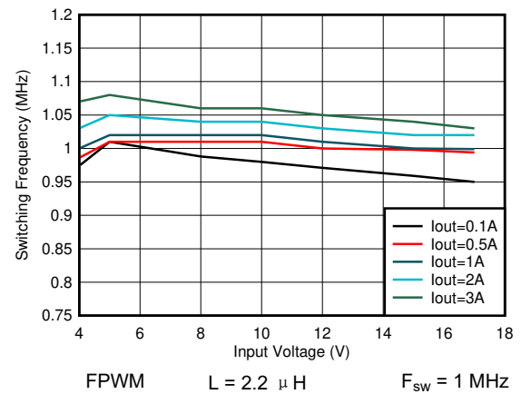
图 8-26. Switching Frequency vs Input Voltage V_{OUT} = 3.3 V
