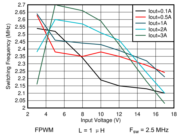
图 8-32. Switching Frequency vs Input Voltage V_{\text{OUT}} = 1.8 \text{ V}
