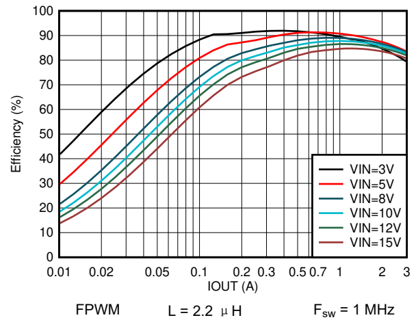
图 8-18. Efficiency vs Output Current V_{OUT} = 1.2 V
