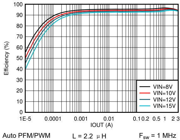
图 8-5. Efficiency vs Output Current V_{\text{OUT}} = 5 \text{ V}
