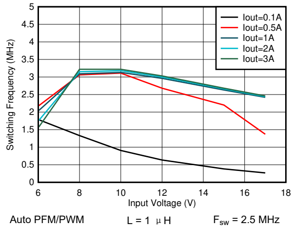
图 8-23. Switching Frequency vs Input Voltage V_{OUT} = 5 V
