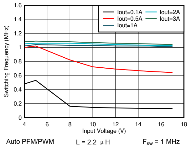
图 8-25. Switching Frequency vs Input Voltage V_{OUT} = 3.3 V
