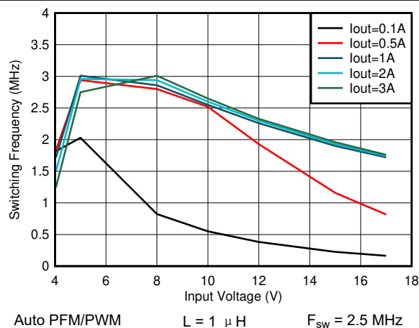
图 8-27. Switching Frequency vs Input Voltage V_{OUT} = 3.3 V
