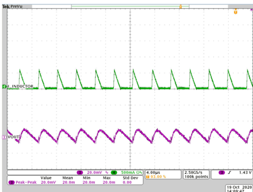
图 8-43. Output Voltage Ripple
