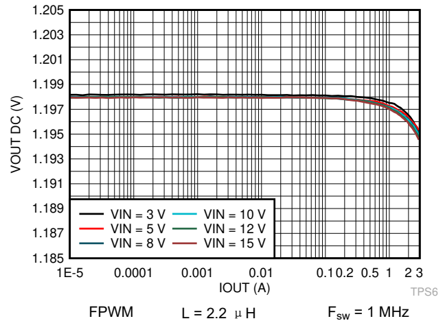
图 8-77. Output Voltage vs Output Current V_{\text{OUT}} = 1.2 \text{ V}
