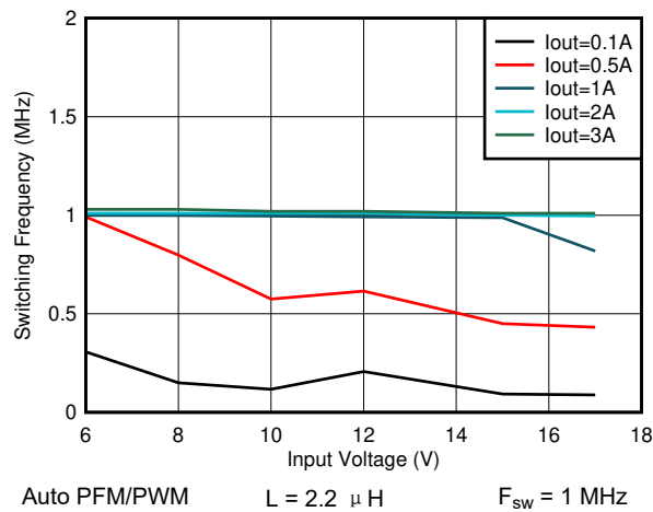
图 8-21. Switching Frequency vs Input Voltage V_{OUT} = 5 V
