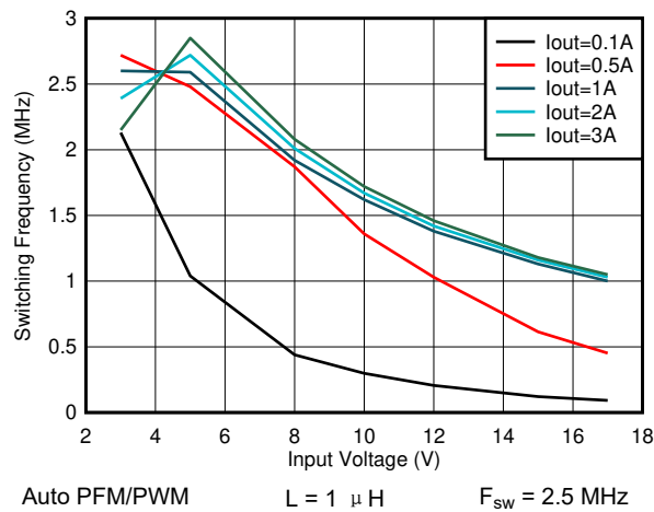
图 8-31. Switching Frequency vs Input Voltage V_{\text{OUT}} = 1.8 \text{ V}
