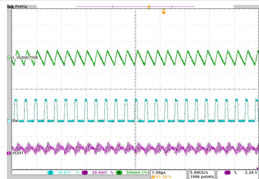
图 8-50. Output Voltage Ripple
