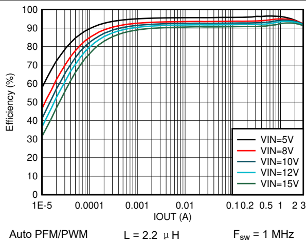
图 8-9. Efficiency vs Output Current V_{\text{OUT}} = 3.3 \text{ V}
