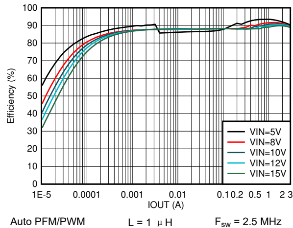
图 8-11. Efficiency vs Output Current V_{\text{OUT}} = 3.3 \text{ V}
