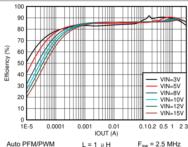
图 8-15. Efficiency vs Output Current V_{\text{OUT}} = 1.8 \text{ V}
