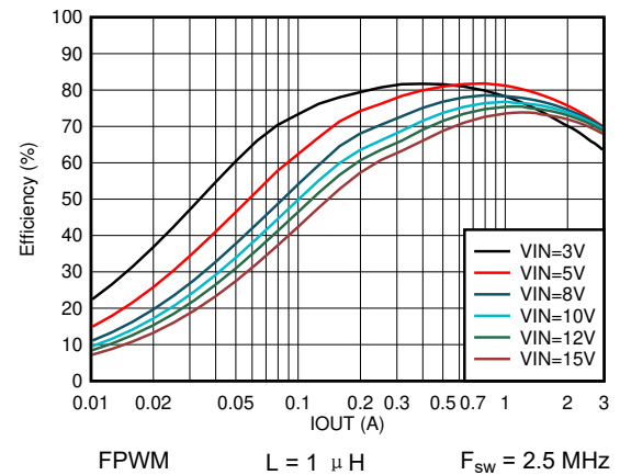
图 8-71. Efficiency vs Output Current V_{OUT} = 0.4\text{ V}
