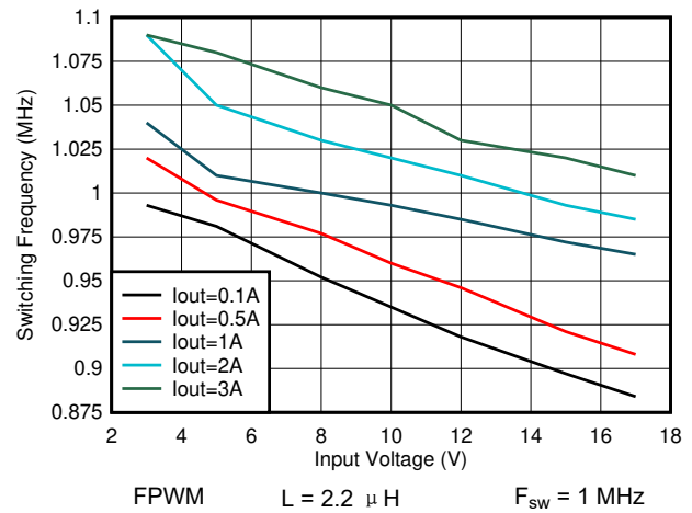
图 8-30. Switching Frequency vs Input Voltage V_{\text{OUT}} = 1.8 \text{ V}
