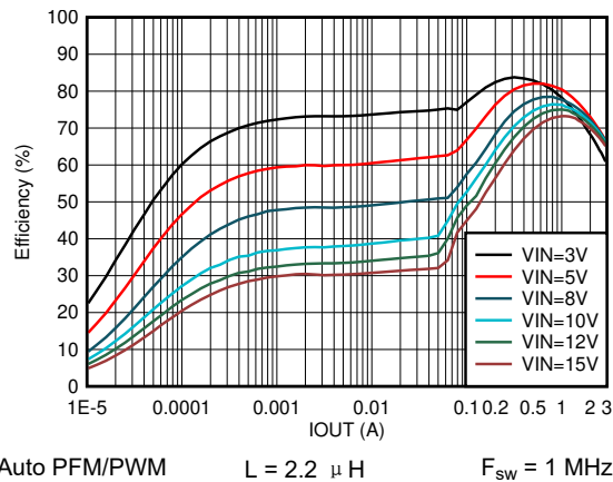
图 8-68. Efficiency vs Output Current V_{OUT} = 0.4\text{ V}
