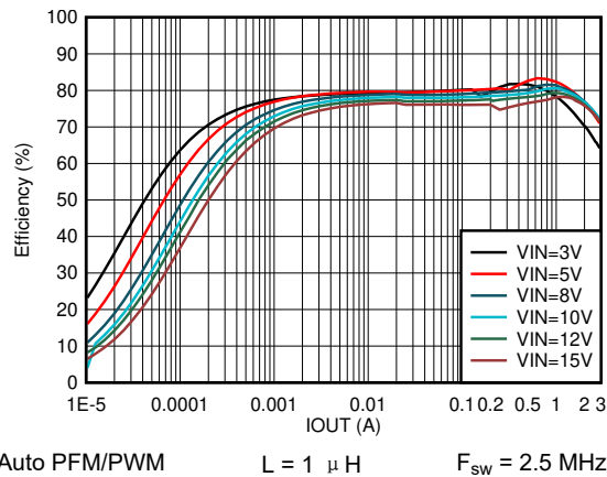
图 8-70. Efficiency vs Output Current V_{OUT} = 0.4\text{ V}
