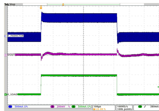
图 8-54. Typical Operation
