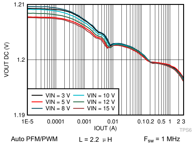
图 8-76. Output Voltage vs Output Current V_{\text{OUT}} = 1.2 \text{ V}
