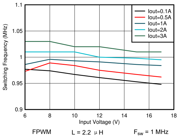
图 8-22. Switching Frequency vs Input Voltage V_{OUT} = 5 V
