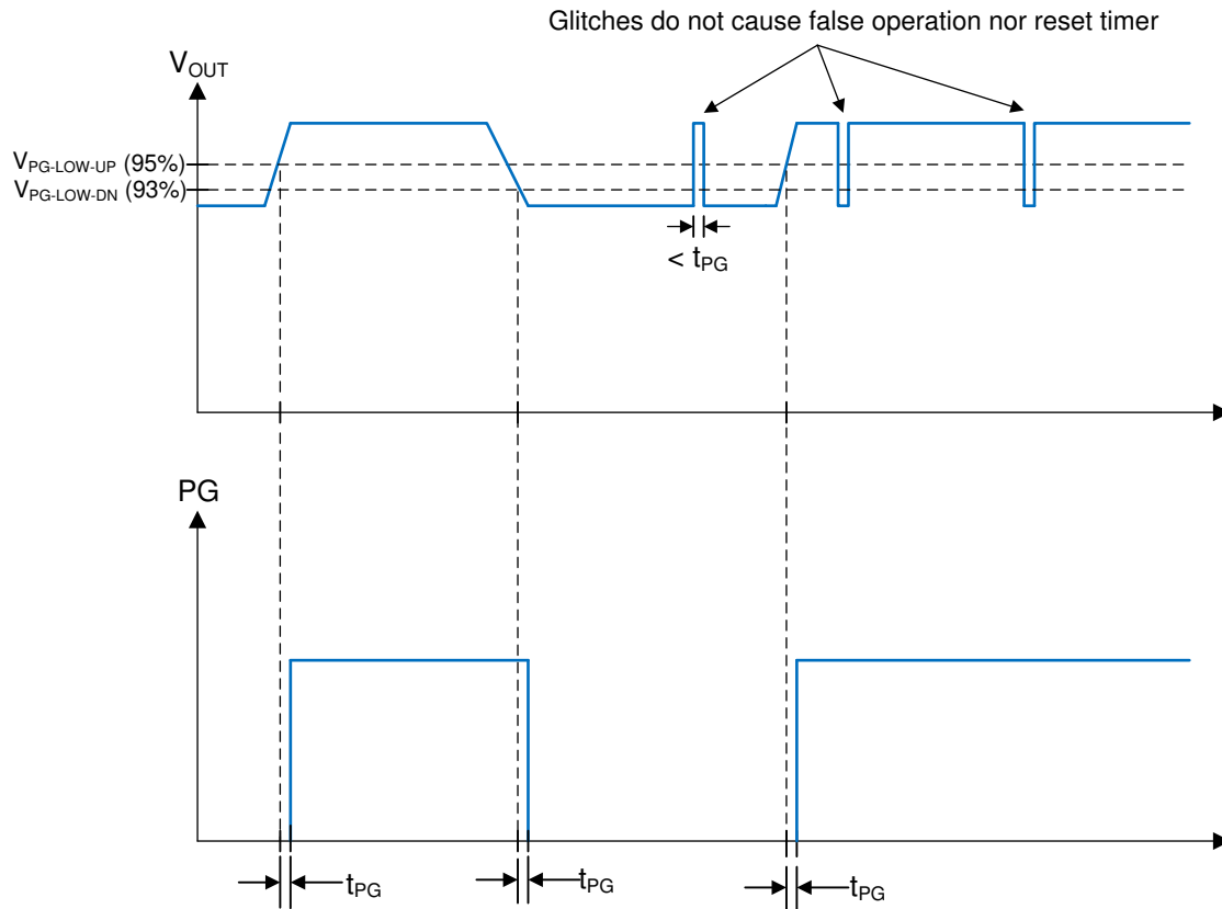
图 8-2. Power-Good-Timing Behavior
