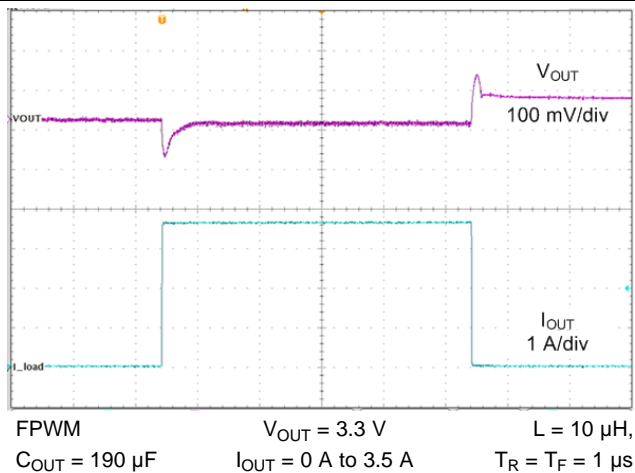
Figure 46. Load Transient
