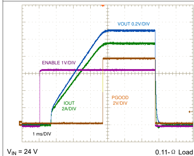
图 9-49. ENABLE ON and OFF, 10-A Resistive Load
