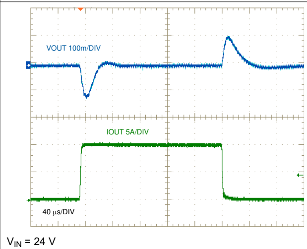
图 9-50. Load Transient Response, 0 A to 10 A to 0 A
