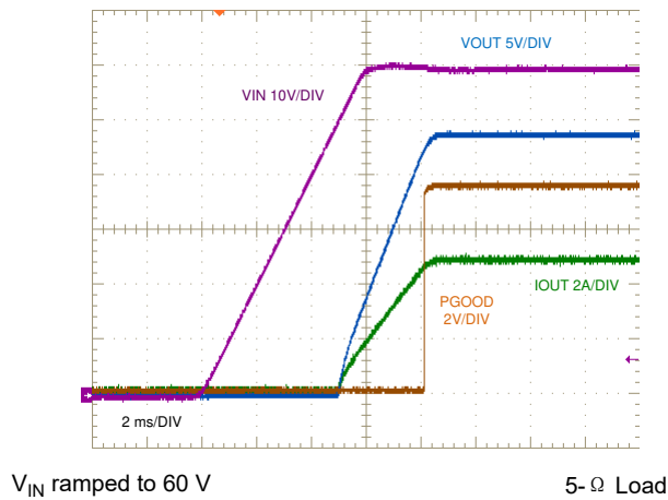
图 9-36. Start-Up, 5-A Resistive Load
