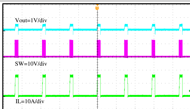
图 32. Transient Response
