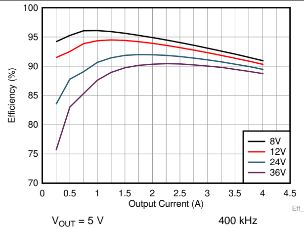
图 12. High-Load Efficiency
