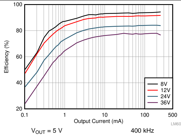
图 11. Low-Load Efficiency
