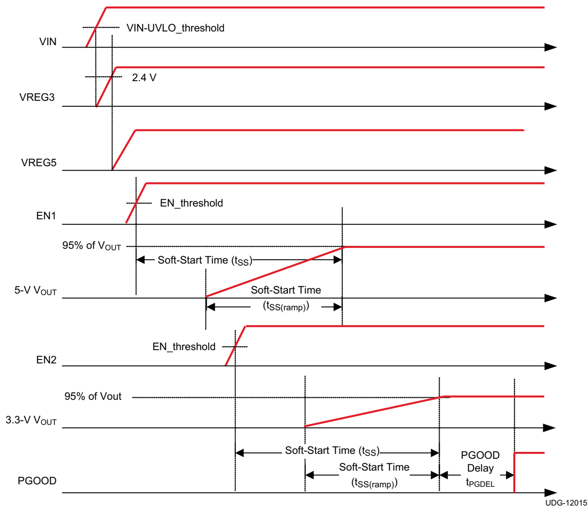
Figure 3. TPS51225C Timing
