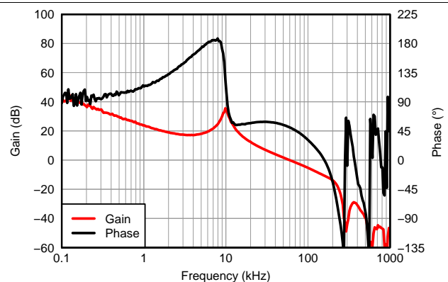
Figure 37. Loop Response
