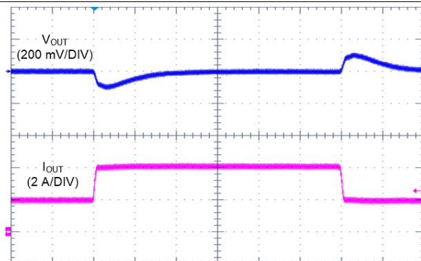
V_{OUT} = 5\text{ V} I_{OUT} = 2\text{ A to } 4\text{ A to } 2\text{ A} Time (20 \mu\text{s}/\text{DIV} ) F_{SW} = 2100\text{ kHz} V_{IN} = 13.5\text{ V} AUTO Mode T_R = T_F = 2\mu\text{s}
