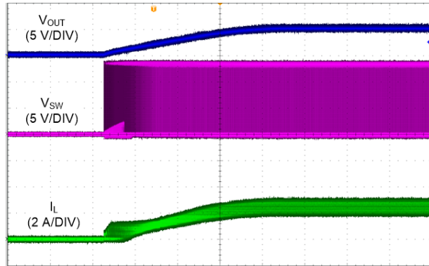
V_{OUT} = 5\text{ V} I_{OUT} = \text{Short Circuit to } 2.5\text{ A} Time (800 \mu\text{s}/\text{DIV} ) F_{SW} = 2100\text{ kHz} V_{IN} = 13.5\text{ V} FPWM Mode
