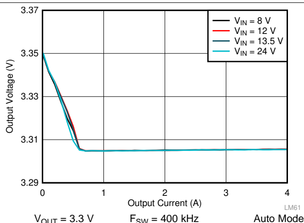
图 38. LM61440-Q1 Load and Line Regulation
