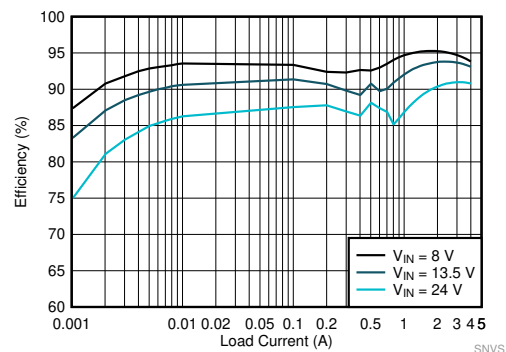
效率: V_{OUT} = 5V , F_{SW} = 2200\text{ kHz}
