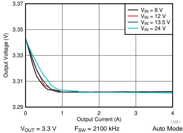
图 40. LM61440-Q1 Load and Line Regulation
