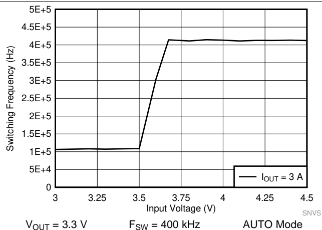
图 50. LM61440-Q1 Frequency Dropout Curve
