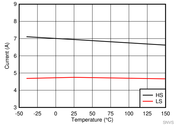
图 4. LM61440-Q1 High-side and Low-side Current Limits
