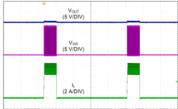
V_{OUT} = 5\text{ V} I_{OUT} = \text{Short Circuit} Time (200 \mu\text{s}/\text{DIV} ) F_{SW} = 2100\text{ kHz} V_{IN} = 13.5\text{ V} FPWM Mode
