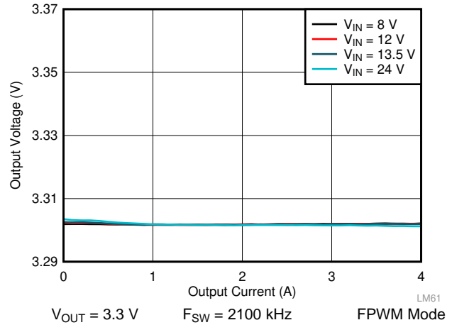
图 41. LM61440-Q1 Load and Line Regulation
