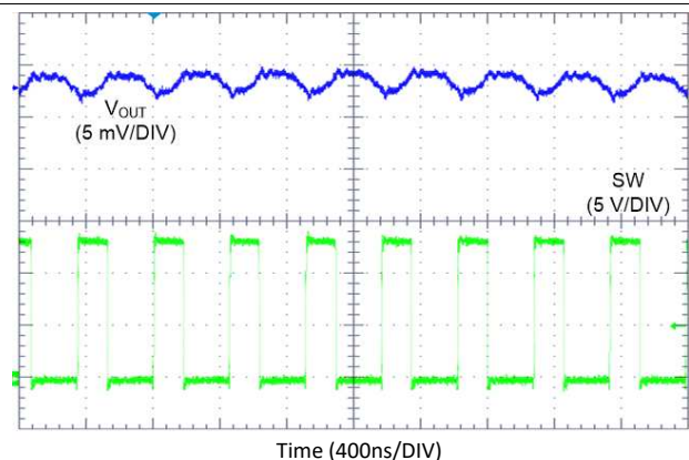
图 55. LM61440-Q1 Switching Waveform and V_{OUT} Ripple
