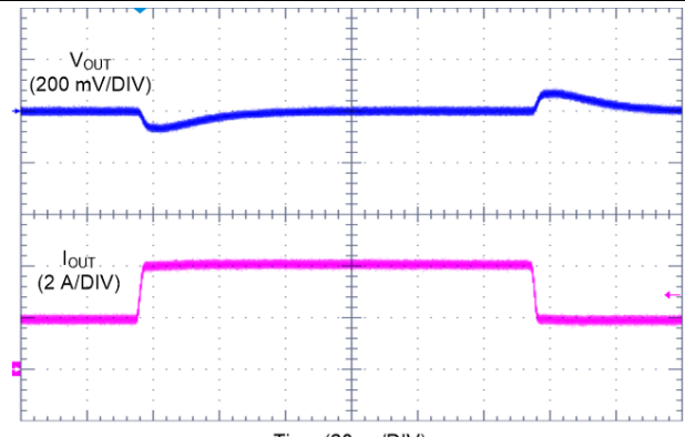
V_{OUT} = 3.3\text{ V} I_{OUT} = 2\text{ A to } 4\text{ A to } 2\text{ A} Time (20 \mu\text{s}/\text{DIV} ) F_{SW} = 2100\text{ kHz} V_{IN} = 13.5\text{ V} AUTO Mode T_R = T_F = 2\mu\text{s}
