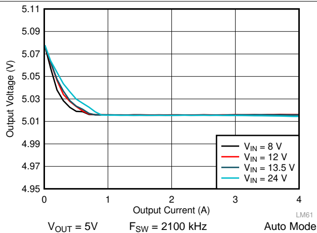
图 44. LM61440-Q1 Load and Line Regulation
