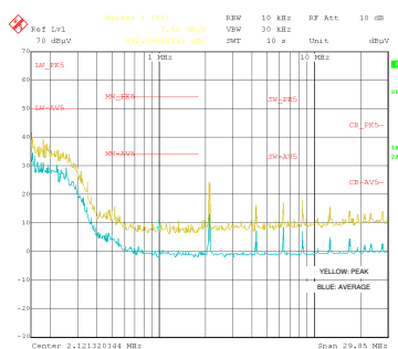
传导 EMI: V_{OUT} = 5V , f_{SW} = 2100\text{kHz}
