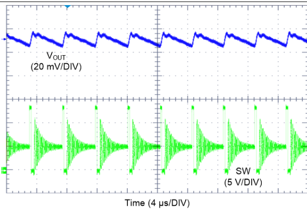
图 54. LM61440-Q1 Switching Waveform and V_{OUT} Ripple
