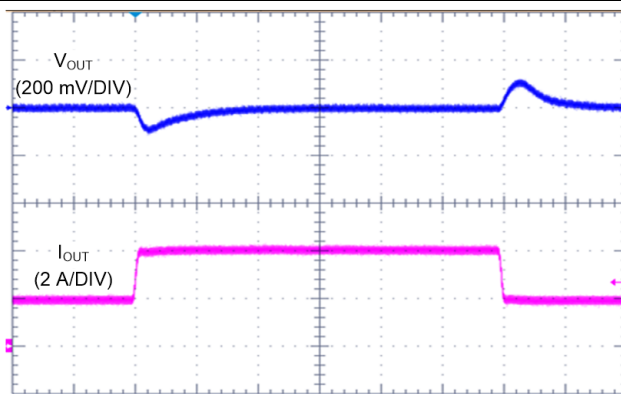
V_{OUT} = 3.3\text{ V} I_{OUT} = 2\text{ A to } 4\text{ A to } 2\text{ A} Time (20 \mu\text{s}/\text{DIV} ) F_{SW} = 400\text{ kHz} V_{IN} = 13.5\text{ V} AUTO Mode T_R = T_F = 2\mu\text{s}
