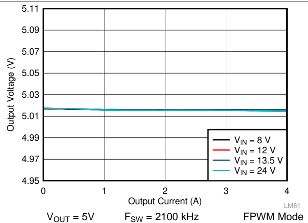
图 45. LM61440-Q1 Load and Line Regulation
