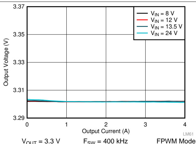
图 39. LM61440-Q1 Load and Line Regulation
