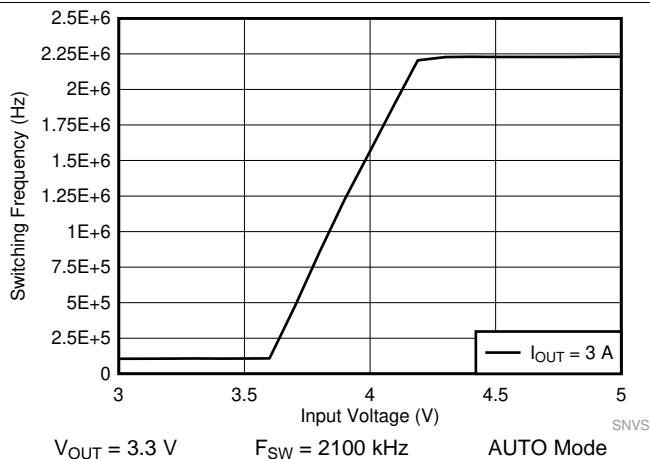
图 51. LM61440-Q1 Frequency Dropout Curve
