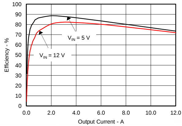
Figure 52. TPS56C20 Efficiency
