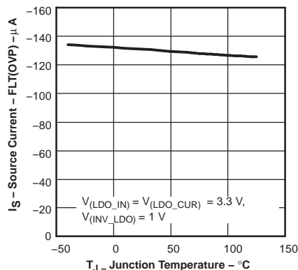
Figure 3. TRIP CURRENT vs JUNCTION TEMPERATURE
