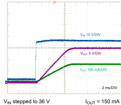
图 8-31. Start-Up, Full Load
