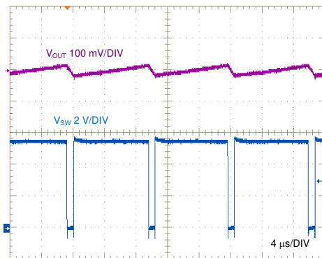
图 8-5. SW Node and Output Ripple Voltage, No Load
