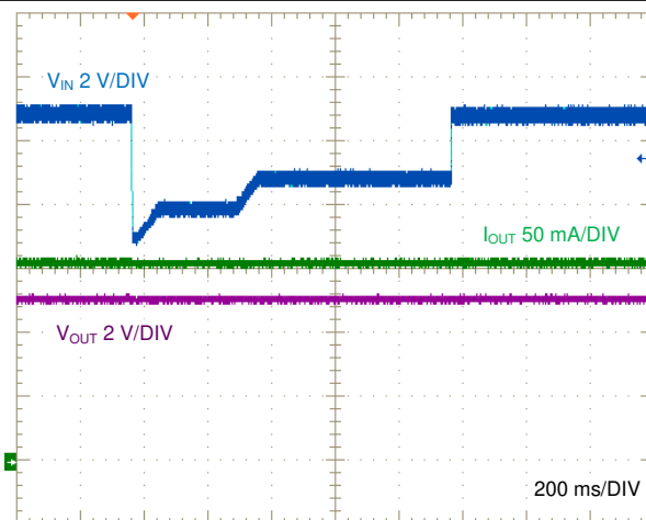
I_{OUT} = 150 mA
