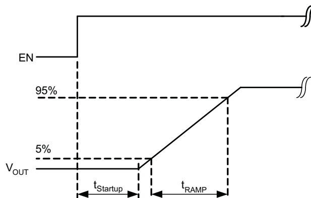
Figure 27. Soft Start
