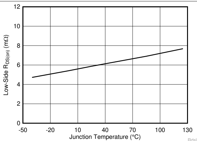
Figure 6-7. Low-Side R_{DS(on)} vs Junction Temperature
