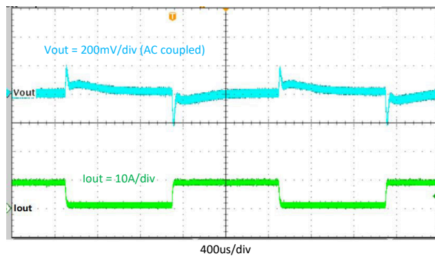
Figure 8-15. Transient Response, 1 A to 9 A, Slew Rate = 2.5\text{ A}/\mu\text{s}
