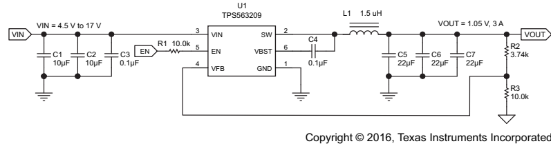
Figure 33. TPS563209 1.05V/3A Reference Design
