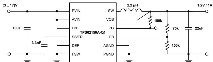
Figure 48. 1.2V/1A Power Supply
