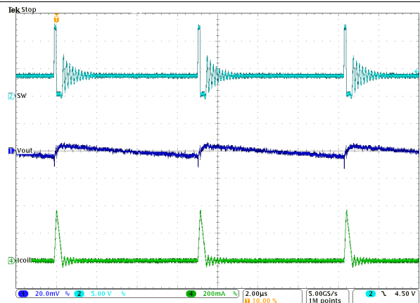
Figure 33. Typical Operation in Power Save Mode ( I_{OUT} = 10mA )
